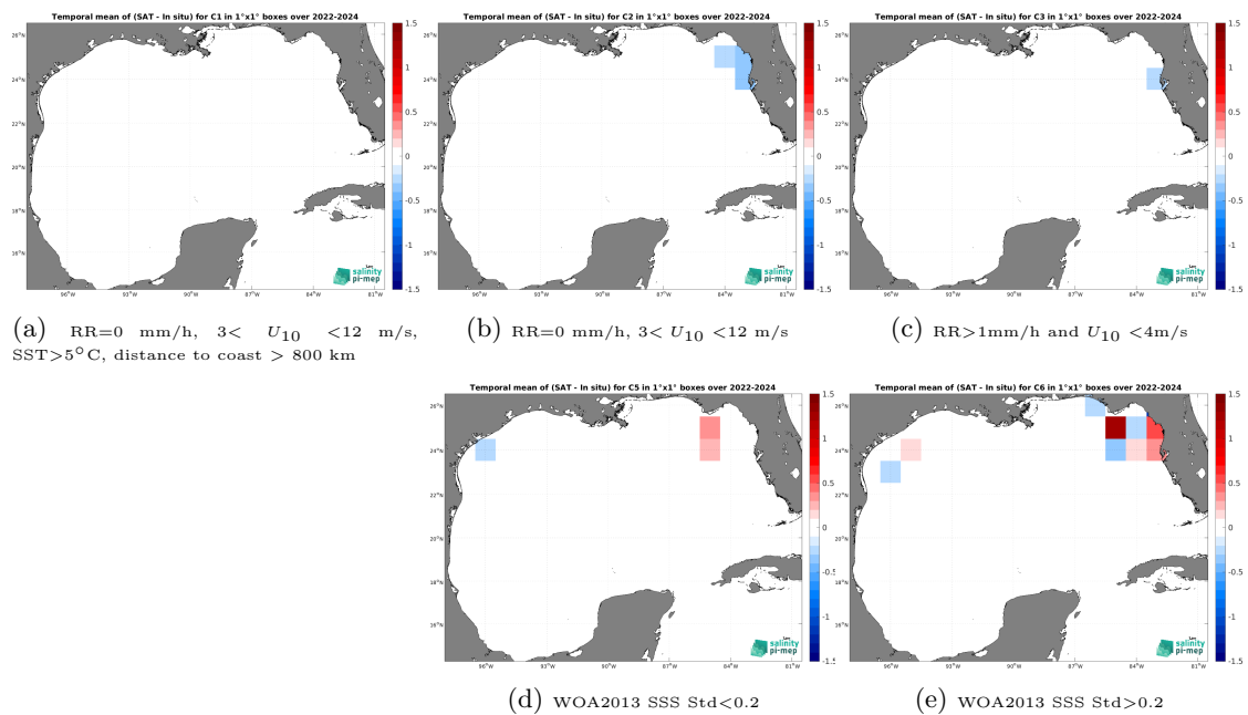
Figure 14: Temporal mean gridded over spatial boxes of size 1^\circ \times 1^\circ of \Delta SSS (SMAP SSS L3 v6 - Monthly (RSS) - Saildrone) for 5 different subdatasets corresponding to:RR=0 mm/h, 3 < U_{10} < 12 m/s, SST >5^\circ C, distance to coast > 800 km (a), RR=0 mm/h, 3 < U_{10} < 12 m/s (b), RR >1 mm/h and U_{10} < 4 m/s (c), WOA2013 SSS Std <0.2 (d), WOA2013 SSS Std >0.2 (e).
