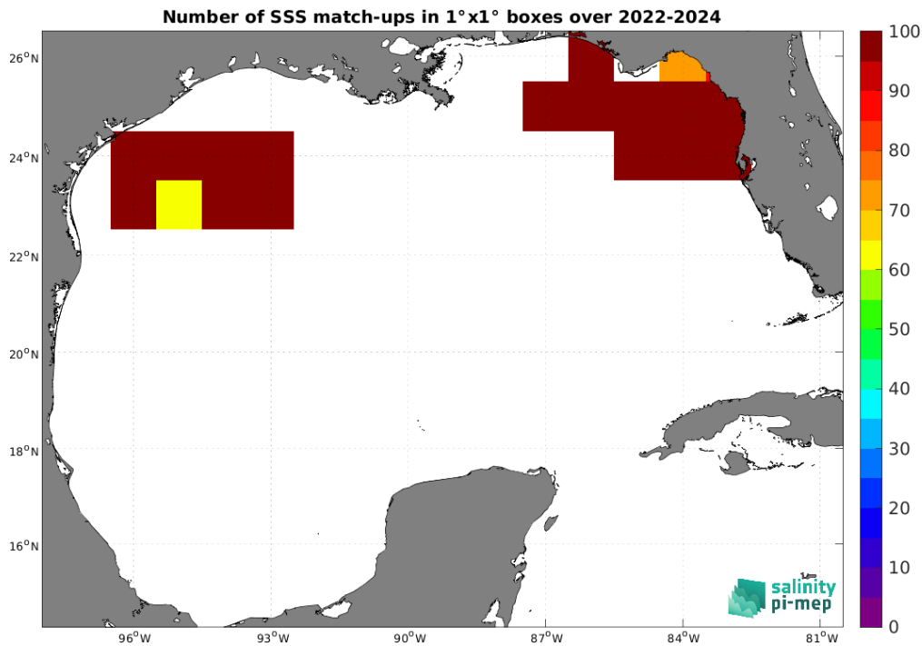
Figure 5: Number of SSS match-ups between Saildrone SSS and the SMAP SSS L3 v6 - Monthly (RSS) SSS product for the Gulf of Mexico Pi-MEP region over 1°×1° boxes and for the full satellite product period.
