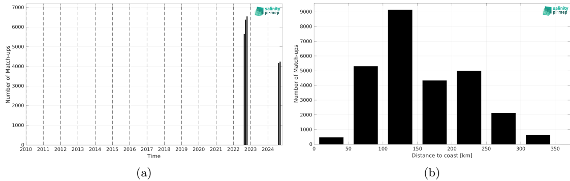
Figure 2: Number of match-ups between Sairdrone and SMAP SSS L3 v6 - Monthly (RSS) SSS as a function of time (a) and as function of the distance to coast (b) over the Gulf of Mexico Pi-MEP region and for the full satellite product period.
