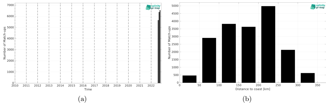
Figure 2: Number of match-ups between Saildrone and SMAP SSS L3 v6 - Monthly (RSS) SSS as a function of time (a) and as function of the distance to coast (b) over the Gulf of Mexico Pi-MEP region and for the full satellite product period.
