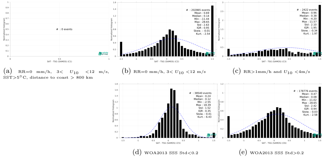
Figure 15: Normalized histogram of \Delta SSS (SMAP SSS L3 v5.3 - 8-Day running (RSS) - TSG (SAMOS)) for 5 different subdatasets corresponding to: RR=0 mm/h, 3 < U_{10} < 12 m/s, SST > 5°C, distance to coast > 800 km (a), RR=0 mm/h, 3 < U_{10} < 12 m/s (b), RR > 1mm/h and U_{10} < 4 m/s (c), WOA2013 SSS Std < 0.2 (d), WOA2013 SSS Std > 0.2 (e).
