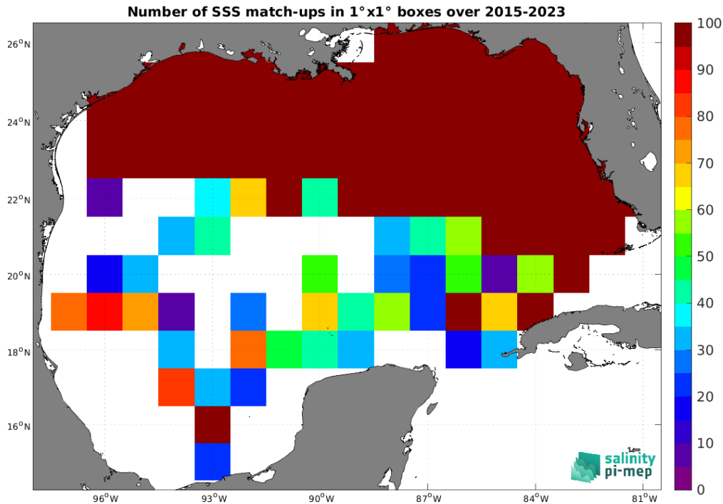
Figure 5: Number of SSS match-ups between TSG (SAMOS) SSS and the SMAP SSS L3 v5.3 - 8-Day running (RSS) SSS product for the Gulf of Mexico Pi-MEP region over 1^\circ \times 1^\circ boxes and for the full satellite product period.
