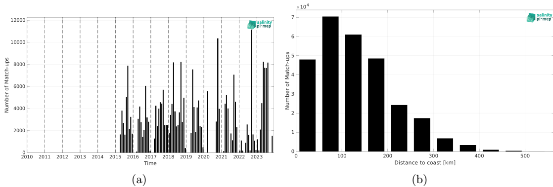
Figure 2: Number of match-ups between TSG (SAMOS) and SMAP SSS L3 v5.3 - 8-Day running (RSS) SSS as a function of time (a) and as function of the distance to coast (b) over the Gulf of Mexico Pi-MEP region and for the full satellite product period.
