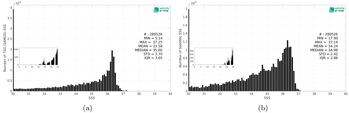
Figure 3: Histograms of SSS from TSG (SAMOS) (a) and SMAP SSS L3 v5.3 - 8-Day running (RSS) (b) considering all match-up pairs per bins of 0.1 over the Gulf of Mexico Pi-MEP region and for the full satellite product period.
