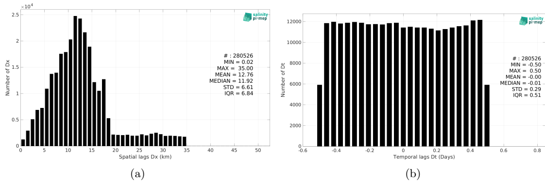
Figure 6: Histograms of the spatial (a) and temporal (b) lags between the location/time of the TSG (SAMOS) measurement and the date of the corresponding SMAP SSS L3 v5.3 - 8-Day running (RSS) SSS pixel.
