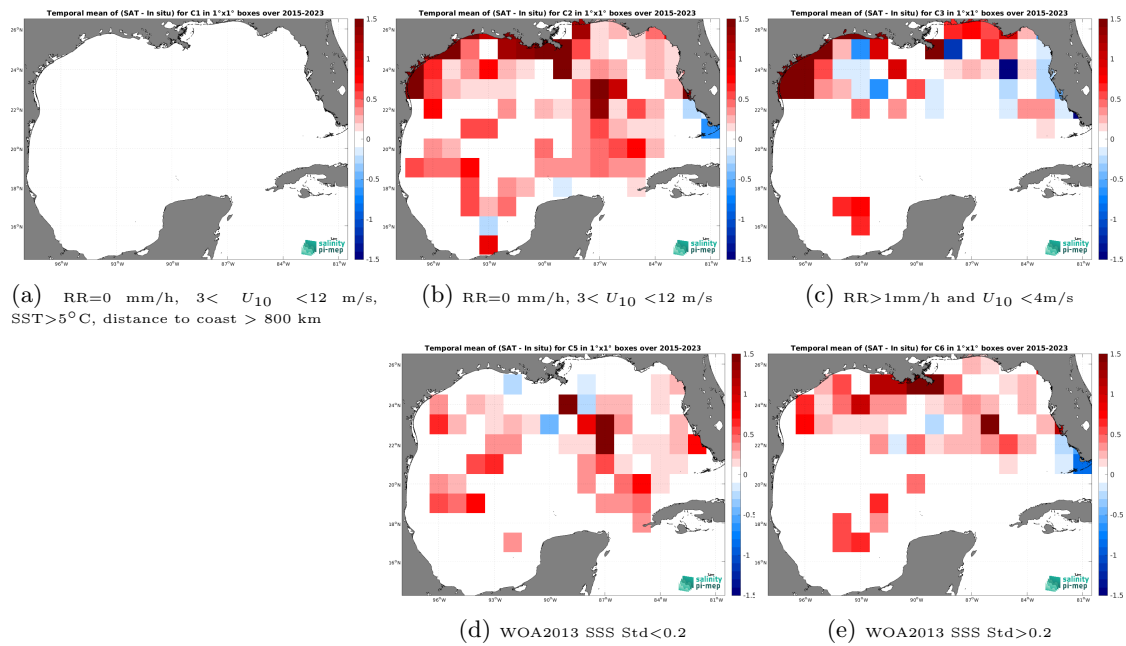
Figure 14: Temporal mean gridded over spatial boxes of size 1^\circ \times 1^\circ of \Delta SSS (SMAP SSS L3 v5.3 - 8-Day running (RSS) - TSG (SAMOS)) for 5 different subdatasets corresponding to:RR=0 mm/h, 3 < U_{10} < 12 m/s, SST > 5^\circ\text{C} , distance to coast > 800 km (a), RR=0 mm/h, 3 < U_{10} < 12 m/s (b), RR > 1 mm/h and U_{10} < 4 m/s (c), WOA2013 SSS Std < 0.2 (d), WOA2013 SSS Std > 0.2 (e).
