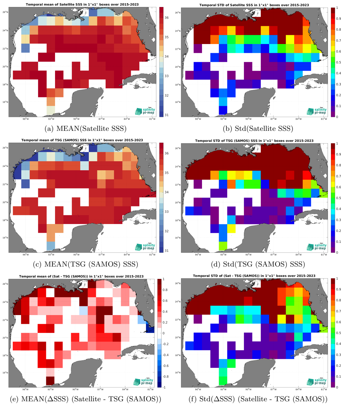
Figure 7: Temporal mean (left) and Std (right) of SSS from SMAP SSS L3 v5.3 - 8-Day running (RSS) (top), TSG (SAMOS) (middle), and of \Delta SSS (Satellite - TSG (SAMOS)). Only match-up pairs are used to generate these maps.
