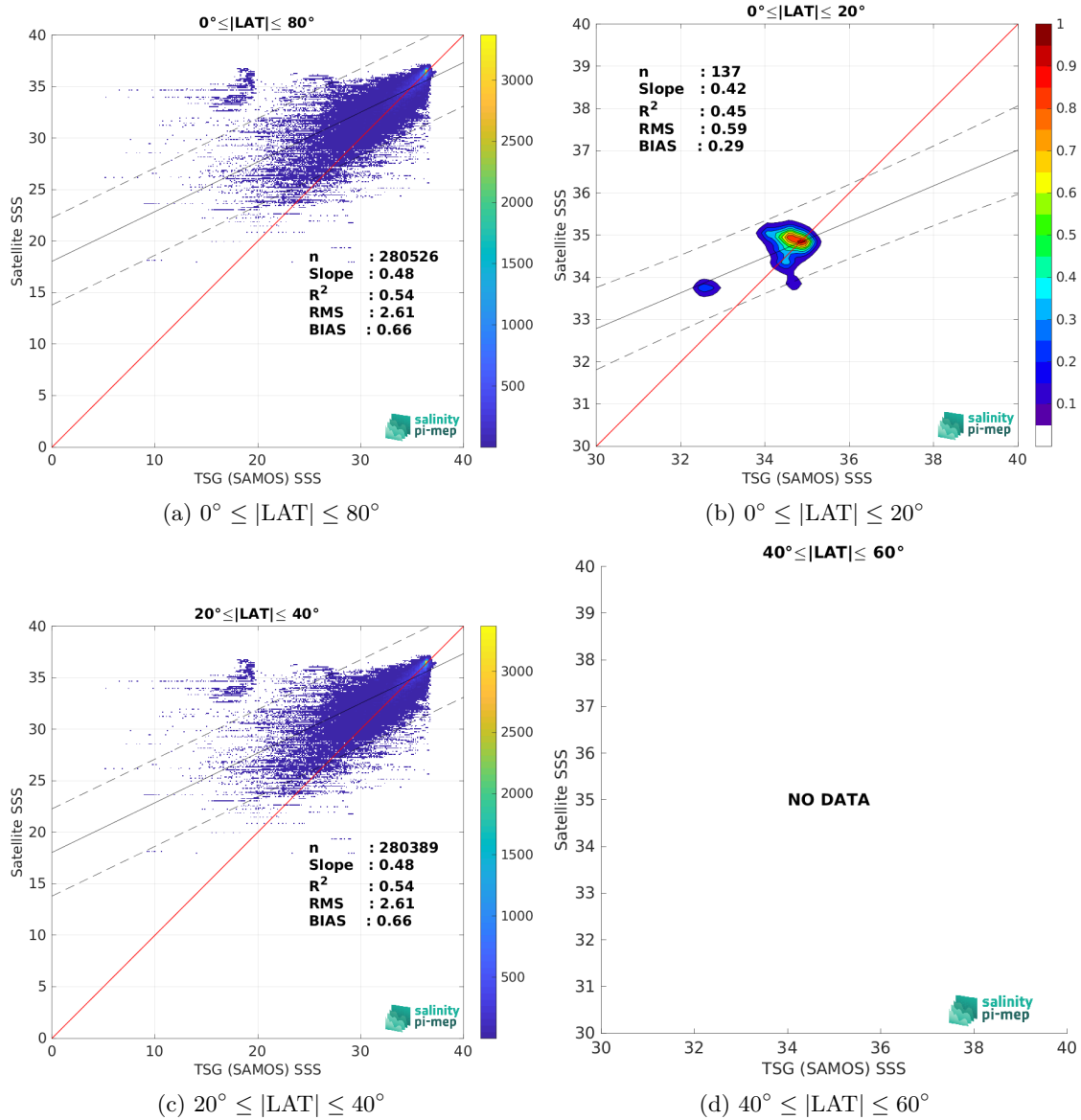
Figure 10: Contour maps of the concentration of SMAP SSS L3 v5.3 - 8-Day running (RSS) SSS (y-axis) versus TSG (SAMOS) SSS (x-axis) at match-up pairs for different latitude bands. For each plot, the red line shows x=y . The black thin and dashed lines indicate a linear fit through the data cloud and the \pm 95\% confidence levels, respectively. The number match-up pairs n , the slope and R^2 coefficient of the linear fit, the root mean square (RMS) and the mean bias between satellite and in situ data are indicated for each latitude band in each plots.
