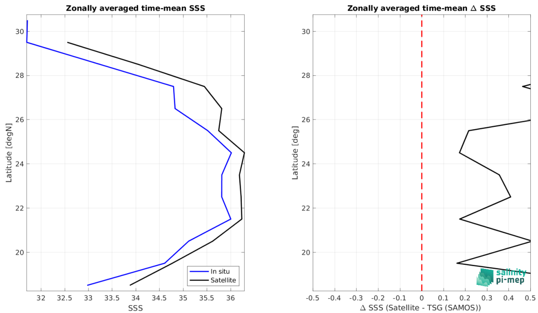
Figure 9: Left panel: Zonal mean SSS from SMAP SSS L3 v5.3 - 8-Day running (RSS) satellite product (black) and from TSG (SAMOS) (blue). Right panel: Zonal mean of \Delta SSS (Satellite - TSG (SAMOS)) for all the collected Pi-MEP match-up pairs estimated over the full satellite product period.
