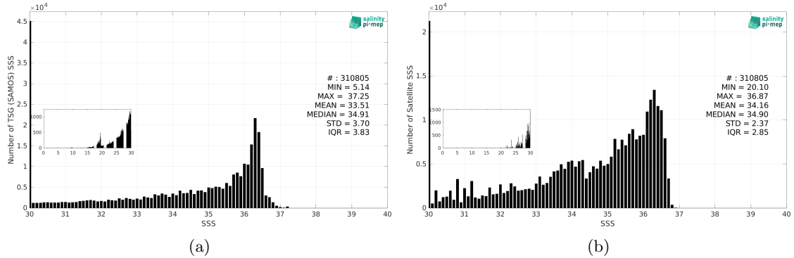
Figure 3: Histograms of SSS from TSG (SAMOS) (a) and SMAP SSS L3 v5.3 - Monthly (RSS) (b) considering all match-up pairs per bins of 0.1 over the Gulf of Mexico Pi-MEP region and for the full satellite product period.
