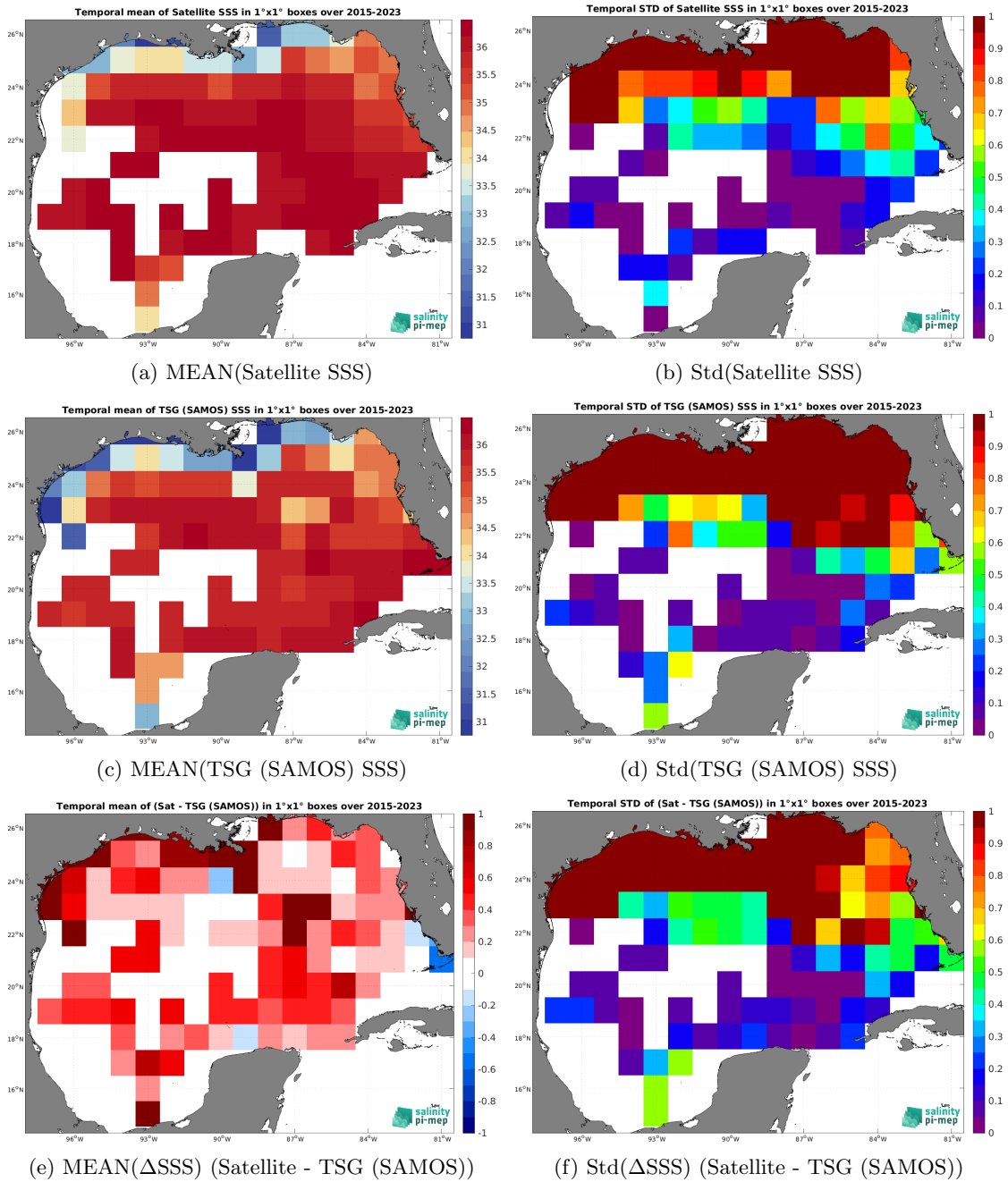
Figure 7: Temporal mean (left) and Std (right) of SSS from SMAP SSS L3 v5.3 - Monthly (RSS) (top), TSG (SAMOS) (middle), and of \Delta SSS (Satellite - TSG (SAMOS)). Only match-up pairs are used to generate these maps.
