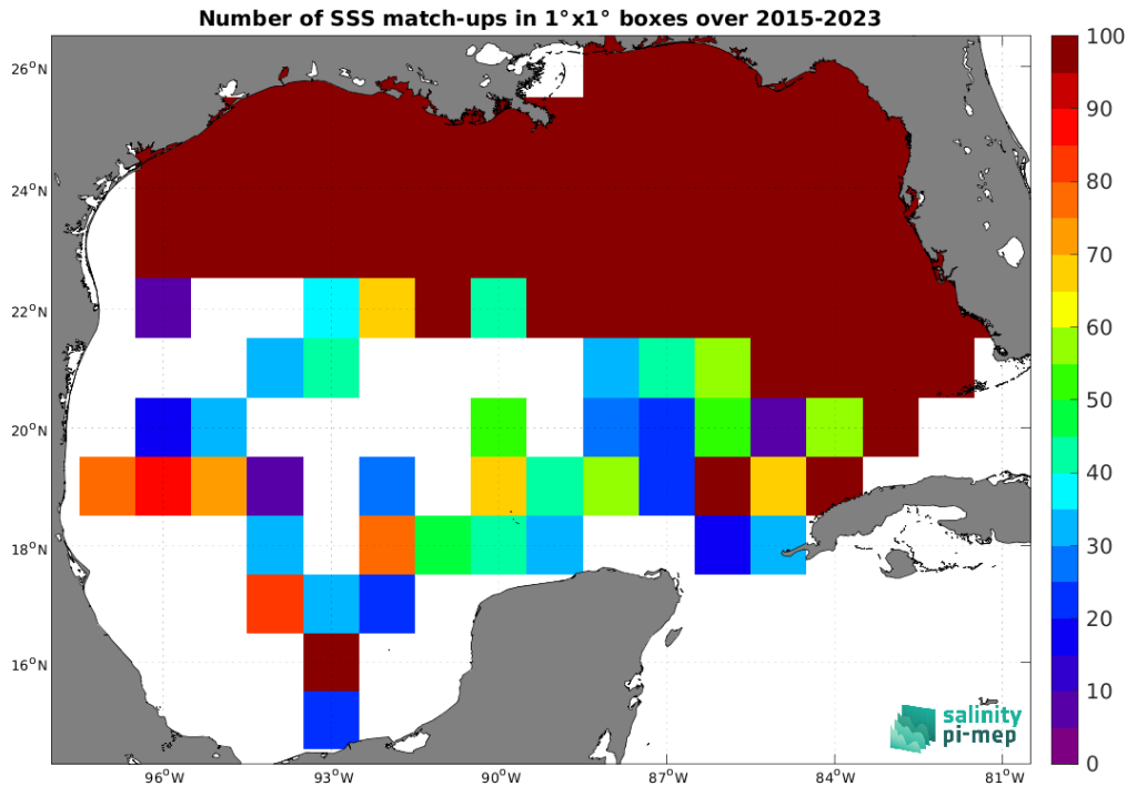
Figure 5: Number of SSS match-ups between TSG (SAMOS) SSS and the SMAP SSS L3 v5.3 - Monthly (RSS) SSS product for the Gulf of Mexico Pi-MEP region over 1^\circ \times 1^\circ boxes and for the full satellite product period.
