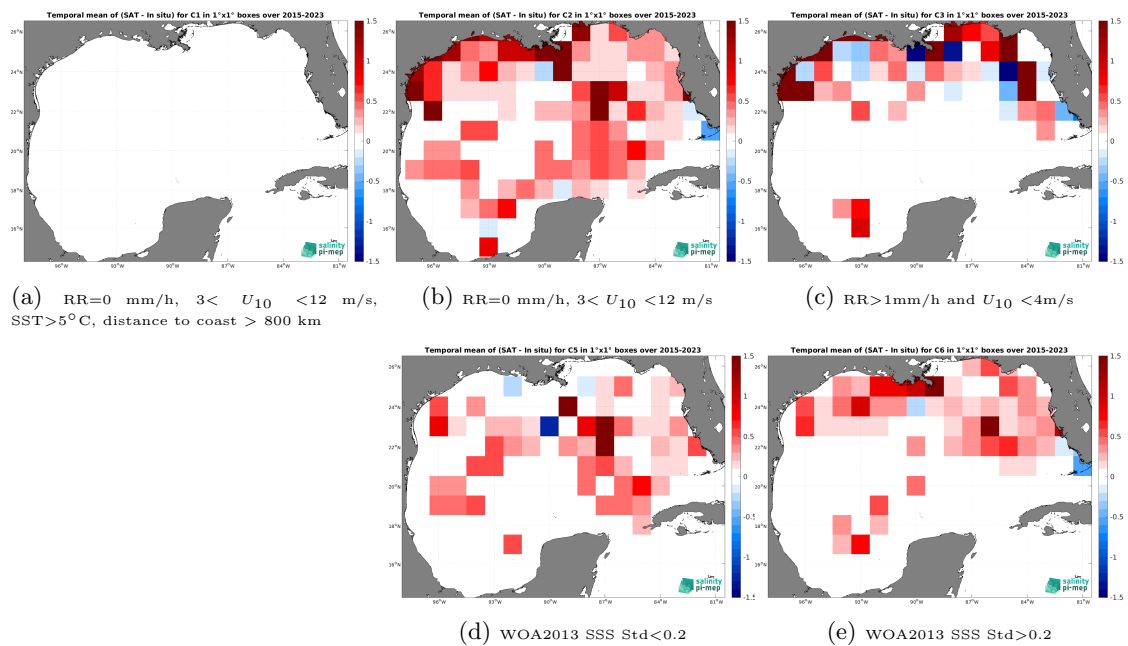
Figure 14: Temporal mean gridded over spatial boxes of size 1^\circ \times 1^\circ of \Delta SSS (SMAP SSS L3 v5.3 - Monthly (RSS) - TSG (SAMOS)) for 5 different subdatasets corresponding to:RR=0 mm/h, 3 < U_{10} < 12 m/s, SST >5^\circ C, distance to coast > 800 km (a), RR=0 mm/h, 3 < U_{10} < 12 m/s (b), RR >1 mm/h and U_{10} < 4 m/s (c), WOA2013 SSS Std <0.2 (d), WOA2013 SSS Std >0.2 (e).
