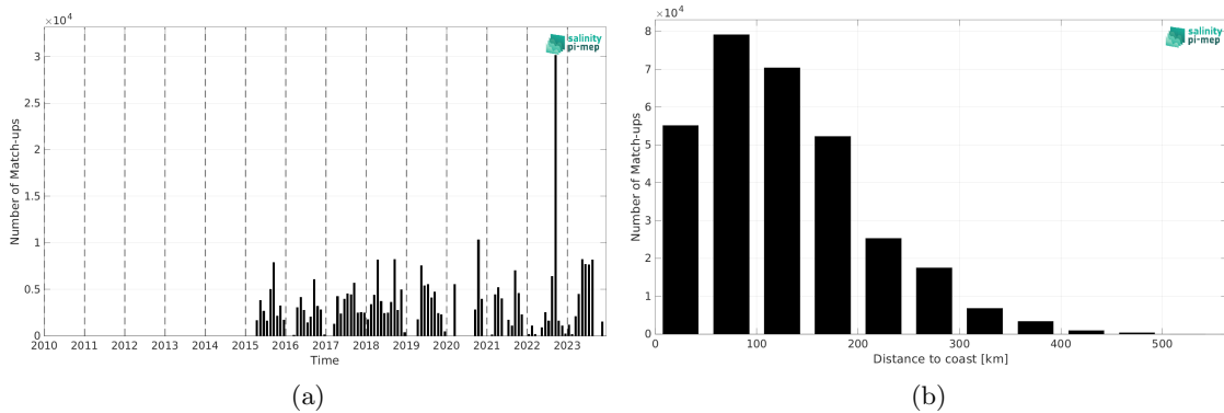
Figure 2: Number of match-ups between TSG (SAMOS) and SMAP SSS L3 v5.3 - Monthly (RSS) SSS as a function of time (a) and as function of the distance to coast (b) over the Gulf of Mexico Pi-MEP region and for the full satellite product period.
