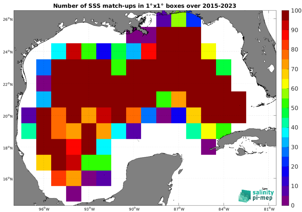
Figure 5: Number of SSS match-ups between Argo SSS and the SMAP SSS L3 v5.3 - Monthly (RSS) SSS product for the Gulf of Mexico Pi-MEP region over 1^\circ \times 1^\circ boxes and for the full satellite product period.
