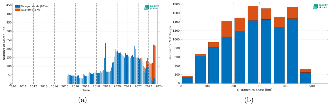
Figure 2: Number of match-ups between Argo and SMAP SSS L3 v5.3 - Monthly (RSS) SSS as a function of time (a) and as function of the distance to coast (b) over the Gulf of Mexico Pi-MEP region and for the full satellite product period.
