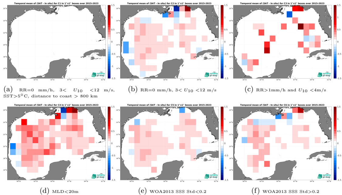
Figure 14: Temporal mean gridded over spatial boxes of size 1^\circ \times 1^\circ of \Delta SSS (SMAP SSS L3 v5.3 - Monthly (RSS) - Argo) for 6 different subdatasets corresponding to:RR=0 mm/h, 3 < U_{10} < 12 m/s, SST > 5^\circ\text{C} , distance to coast > 800 km (a), RR=0 mm/h, 3 < U_{10} < 12 m/s (b), RR > 1 mm/h and U_{10} < 4 m/s (c),MLD < 20 m (d),WOA2013 SSS Std < 0.2 (e),WOA2013 SSS Std > 0.2 (f).
