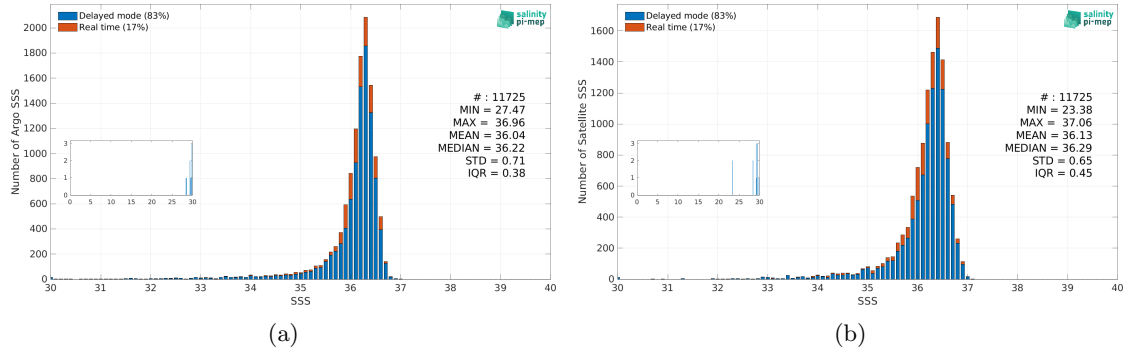
Figure 3: Histograms of SSS from Argo (a) and SMAP SSS L3 v5.3 - Monthly (RSS) (b) considering all match-up pairs per bins of 0.1 over the Gulf of Mexico Pi-MEP region and for the full satellite product period.
