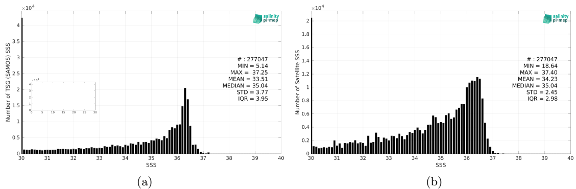
Figure 2: Histograms of SSS from TSG (SAMOS) (a) and SMAP SSS L3 v5 - 8-Day running (RSS) (b) considering all match-up pairs per bins of 0.1 over the Gulf of Mexico Pi-MEP region and for the full satellite product period.
