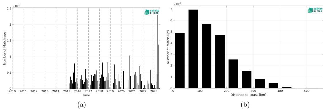
Figure 1: Number of match-ups between TSG (SAMOS) and SMAP SSS L3 v5 - 8-Day running (RSS) SSS as a function of time (a) and as function of the distance to coast (b) over the Gulf of Mexico Pi-MEP region and for the full satellite product period.
