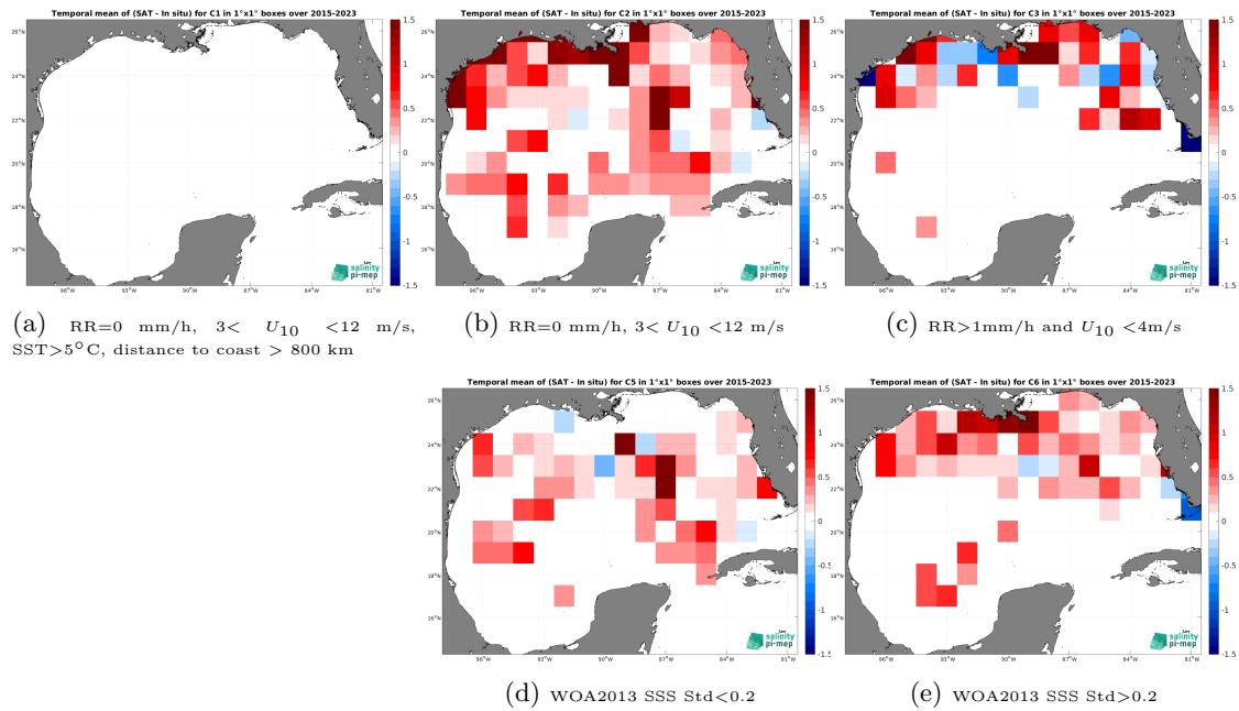
Figure 12: Temporal mean gridded over spatial boxes of size 1^\circ \times 1^\circ of \Delta SSS (SMAP SSS L3 v5 - 8-Day running (RSS) - TSG (SAMOS)) for 5 different subdatasets corresponding to:RR=0 mm/h, 3 < U_{10} < 12 m/s, SST > 5^\circ\text{C} , distance to coast > 800 km (a), RR=0 mm/h, 3 < U_{10} < 12 m/s (b), RR > 1 mm/h and U_{10} < 4 m/s (c), WOA2013 SSS Std < 0.2 (d), WOA2013 SSS Std > 0.2 (e).
