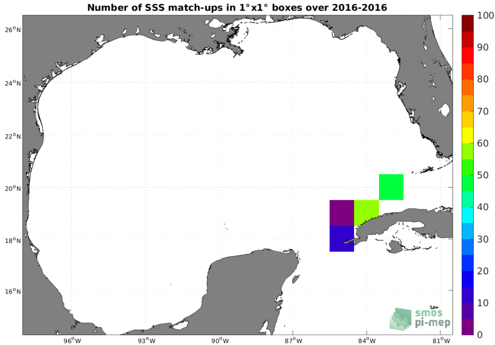
Figure 4: Number of SSS match-ups between TSG (LEGOS-DM) SSS and the SMAP SSS L3 v5 - 8-Day running (RSS) SSS product for the Gulf of Mexico Pi-MEP region over 1^\circ \times 1^\circ boxes and for the full satellite product period.
