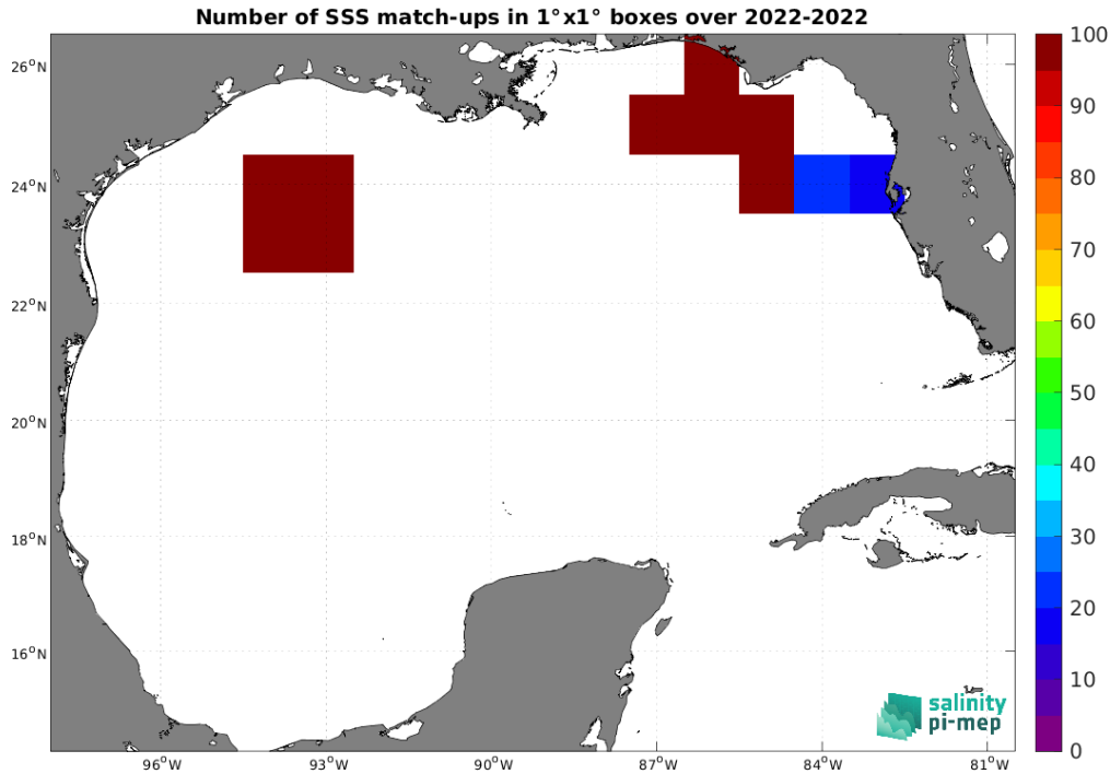
Figure 4: Number of SSS match-ups between Saildrone SSS and the SMAP SSS L3 v5 - 8-Day running (RSS) SSS product for the Gulf of Mexico Pi-MEP region over 1^{\circ} \times 1^{\circ} boxes and for the full satellite product period.
