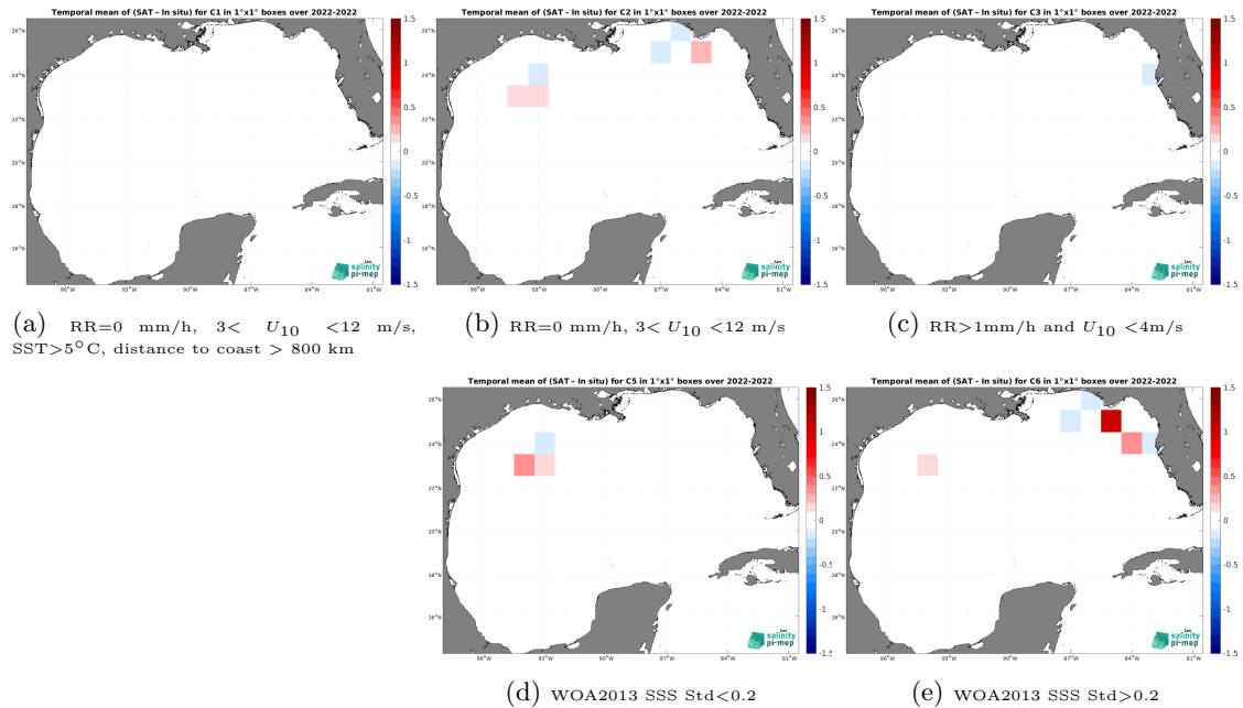
Figure 12: Temporal mean gridded over spatial boxes of size 1^{\circ}\times 1^{\circ} of \Delta\text{SSS} (SMAP SSS L3 v5 - 8-Day running (RSS) - Saildrone) for 5 different subdatasets corresponding to:RR=0 mm/h, 3 < U_{10} < 12 m/s, SST >5^{\circ}\text{C} , distance to coast > 800 km (a), RR=0 mm/h, 3 < U_{10} < 12 m/s (b), RR >1 mm/h and U_{10} < 4 m/s (c), WOA2013 SSS Std <0.2 (d), WOA2013 SSS Std >0.2 (e).
