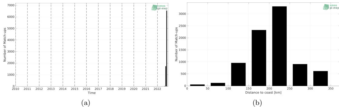
Figure 1: Number of match-ups between Saildrone and SMAP SSS L3 v5 - 8-Day running (RSS) SSS as a function of time (a) and as function of the distance to coast (b) over the Gulf of Mexico Pi-MEP region and for the full satellite product period.
