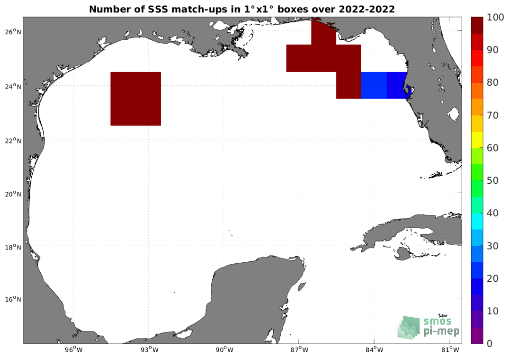
Figure 4: Number of SSS match-ups between Saildrone SSS and the SMAP SSS L3 v5 - 8-Day running (RSS) SSS product for the Gulf of Mexico Pi-MEP region over 1^\circ \times 1^\circ boxes and for the full satellite product period.
