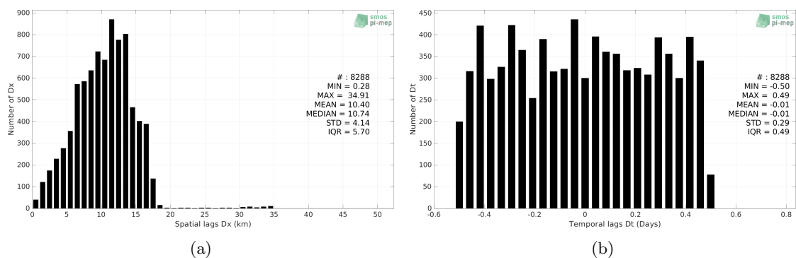
Figure 5: Histograms of the spatial (a) and temporal (b) lags between the location/time of the Saildrone measurement and the date of the corresponding SMAP SSS L3 v5 - 8-Day running (RSS) SSS pixel.
