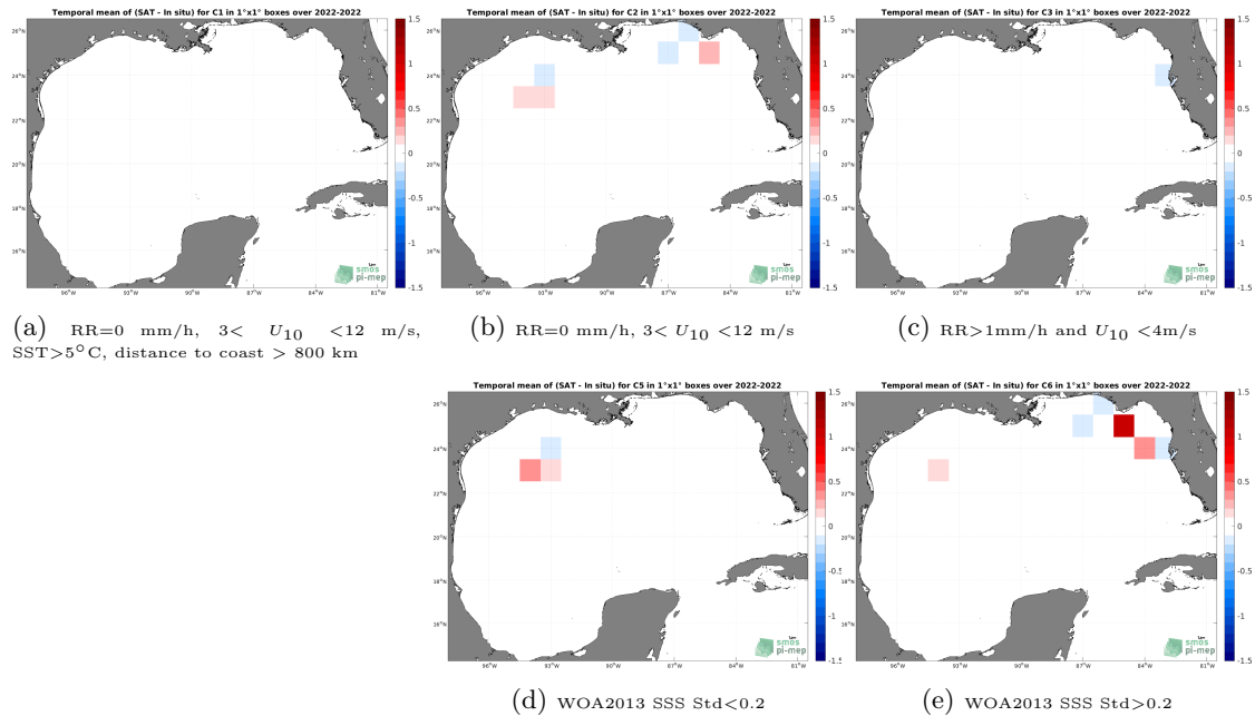
Figure 12: Temporal mean gridded over spatial boxes of size 1^{\circ}\times 1^{\circ} of \Delta\text{SSS} (SMAP SSS L3 v5 - 8-Day running (RSS) - Sairdrone) for 5 different subdatasets corresponding to:RR=0 mm/h, 3 < U_{10} < 12 m/s, SST >5^{\circ}\text{C} , distance to coast > 800 km (a), RR=0 mm/h, 3 < U_{10} < 12 m/s (b), RR >1 mm/h and U_{10} < 4 m/s (c), WOA2013 SSS Std <0.2 (d), WOA2013 SSS Std >0.2 (e).
