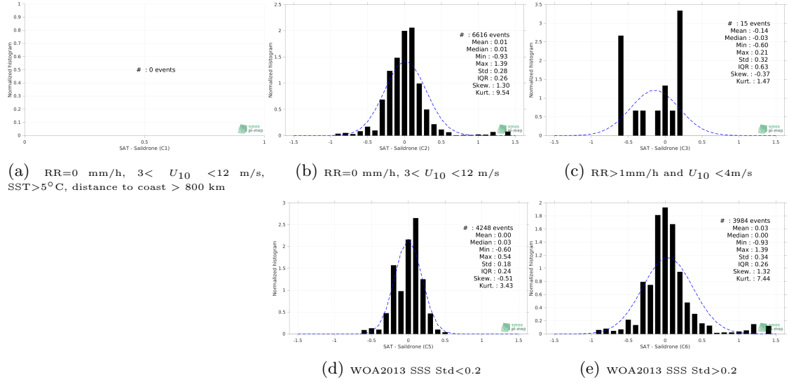
Figure 13: Normalized histogram of \Delta SSS (SMAP SSS L3 v5 - 8-Day running (RSS) - Saldrone) for 5 different subdatasets corresponding to: RR=0 mm/h, 3 < U_{10} < 12 m/s, SST > 5°C, distance to coast > 800 km (a), RR=0 mm/h, 3 < U_{10} < 12 m/s (b), RR > 1mm/h and U_{10} < 4 m/s (c), WOA2013 SSS Std < 0.2 (d), WOA2013 SSS Std > 0.2 (e).
