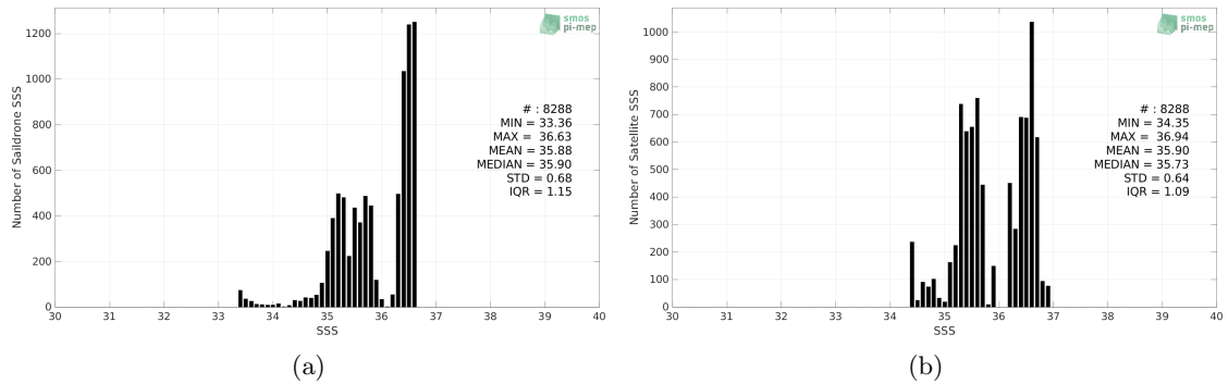
Figure 2: Histograms of SSS from Saildrone (a) and SMAP SSS L3 v5 - 8-Day running (RSS) (b) considering all match-up pairs per bins of 0.1 over the Gulf of Mexico Pi-MEP region and for the full satellite product period.
