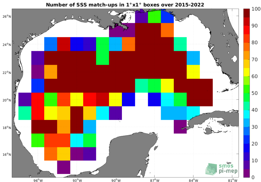
Figure 4: Number of SSS match-ups between Argo SSS and the SMAP SSS L3 v5 - 8-Day running (RSS) SSS product for the Gulf of Mexico Pi-MEP region over 1^\circ \times 1^\circ boxes and for the full satellite product period.
