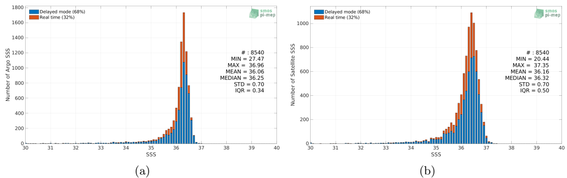
Figure 2: Histograms of SSS from Argo (a) and SMAP SSS L3 v5 - 8-Day running (RSS) (b) considering all match-up pairs per bins of 0.1 over the Gulf of Mexico Pi-MEP region and for the full satellite product period.
