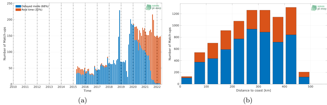
Figure 1: Number of match-ups between Argo and SMAP SSS L3 v5 - 8-Day running (RSS) SSS as a function of time (a) and as function of the distance to coast (b) over the Gulf of Mexico Pi-MEP region and for the full satellite product period.
