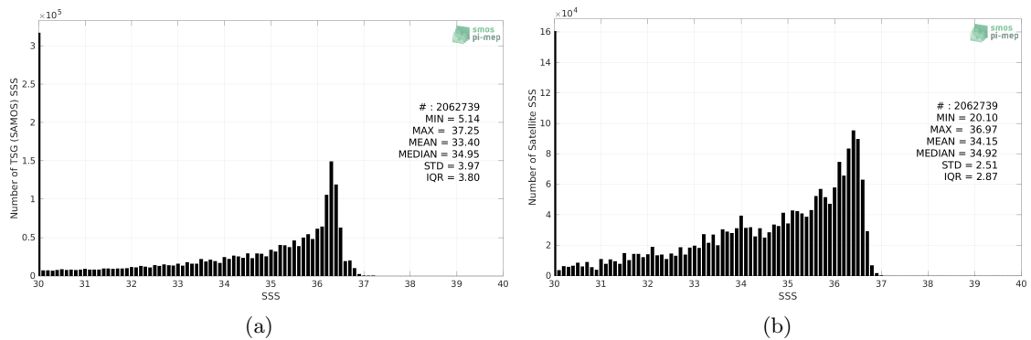
Figure 2: Histograms of SSS from TSG (SAMOS) (a) and SMAP SSS L3 v5 - Monthly (RSS) (b) considering all match-up pairs per bins of 0.1 over the Gulf of Mexico Pi-MEP region and for the full satellite product period.
