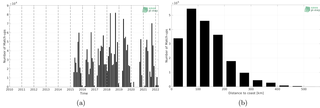
Figure 1: Number of match-ups between TSG (SAMOS) and SMAP SSS L3 v5 - Monthly (RSS) SSS as a function of time (a) and as function of the distance to coast (b) over the Gulf of Mexico Pi-MEP region and for the full satellite product period.
