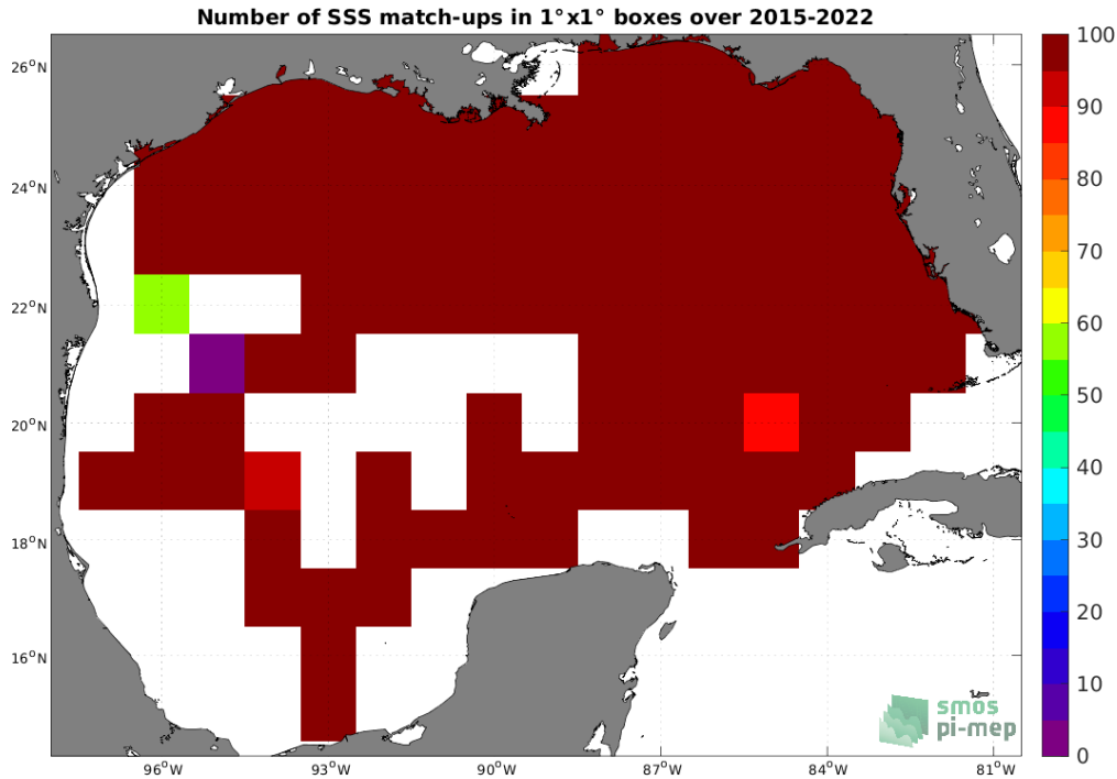
Figure 4: Number of SSS match-ups between TSG (SAMOS) SSS and the SMAP SSS L3 v5 - Monthly (RSS) SSS product for the Gulf of Mexico Pi-MEP region over 1^\circ \times 1^\circ boxes and for the full satellite product period.
