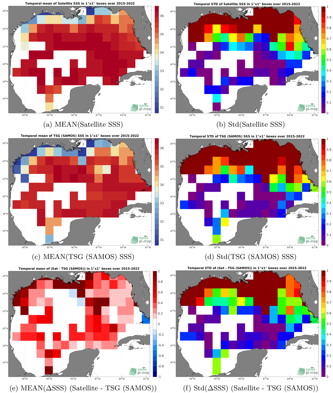
Figure 6: Temporal mean (left) and Std (right) of SSS from SMAP SSS L3 v5 - Monthly (RSS) (top), TSG (SAMOS) (middle), and of \Delta SSS (Satellite - TSG (SAMOS)). Only match-up pairs are used to generate these maps.
