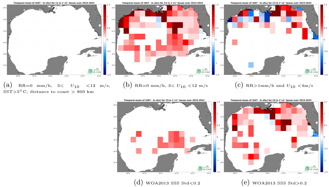
Figure 12: Temporal mean gridded over spatial boxes of size 1^\circ \times 1^\circ of \Delta SSS (SMAP SSS L3 v5 - Monthly (RSS) - TSG (SAMOS)) for 5 different subdatasets corresponding to:RR=0 mm/h, 3 < U_{10} < 12 m/s, SST >5^\circ\text{C} , distance to coast > 800 km (a), RR=0 mm/h, 3 < U_{10} < 12 m/s (b), RR >1 mm/h and U_{10} < 4 m/s (c), WOA2013 SSS Std <0.2 (d), WOA2013 SSS Std >0.2 (e).
