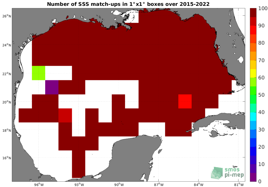
Figure 4: Number of SSS match-ups between TSG (SAMOS) SSS and the SMAP SSS L3 v5 - Monthly (RSS) SSS product for the Gulf of Mexico Pi-MEP region over 1°x1° boxes and for the full satellite product period.
