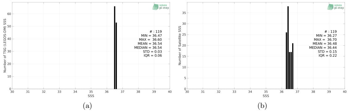
Figure 2: Histograms of SSS from TSG (LEGOS-DM) (a) and SMAP SSS L3 v5 - Monthly (RSS) (b) considering all match-up pairs per bins of 0.1 over the Gulf of Mexico Pi-MEP region and for the full satellite product period.
