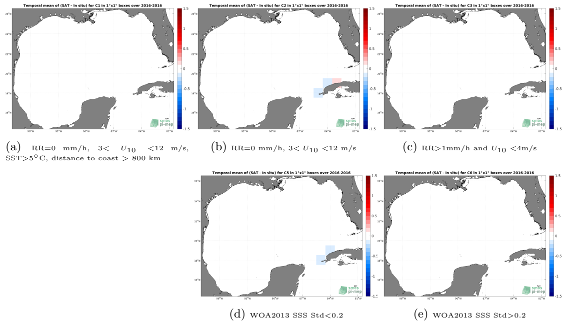
Figure 12: Temporal mean gridded over spatial boxes of size 1^{\circ}\times 1^{\circ} of \Delta\text{SSS} (SMAP SSS L3 v5 - Monthly (RSS) - TSG (LEGOS-DM)) for 5 different subdatasets corresponding to:RR=0 mm/h, 3 < U_{10} < 12 m/s, SST >5^{\circ}\text{C} , distance to coast > 800 km (a), RR=0 mm/h, 3 < U_{10} < 12 m/s (b), RR >1 mm/h and U_{10} < 4 m/s (c), WOA2013 SSS Std <0.2 (d), WOA2013 SSS Std >0.2 (e).
