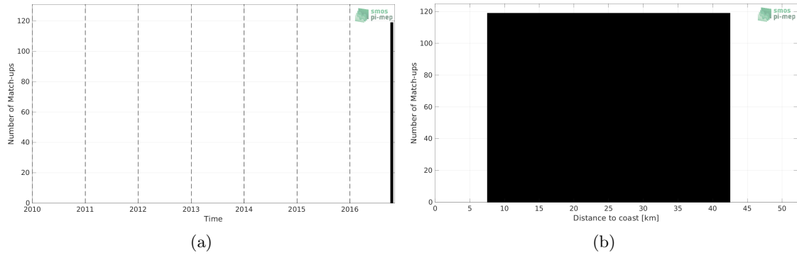
Figure 1: Number of match-ups between TSG (LEGOS-DM) and SMAP SSS L3 v5 - Monthly (RSS) SSS as a function of time (a) and as function of the distance to coast (b) over the Gulf of Mexico Pi-MEP region and for the full satellite product period.
