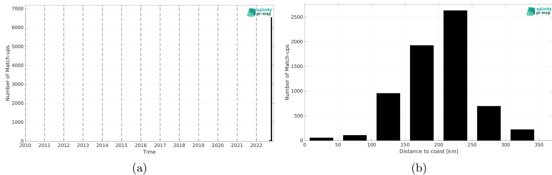
Figure 1: Number of match-ups between Saildrone and SMAP SSS L3 v5 - Monthly (RSS) SSS as a function of time (a) and as function of the distance to coast (b) over the Gulf of Mexico Pi-MEP region and for the full satellite product period.
