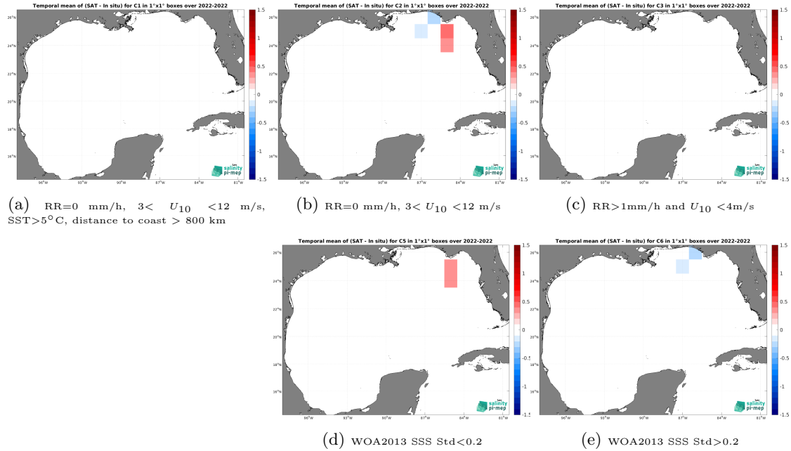
Figure 12: Temporal mean gridded over spatial boxes of size 1^{\circ}\times 1^{\circ} of \Delta\text{SSS} (SMAP SSS L3 v5 - Monthly (RSS) - Saildrone) for 5 different subdatasets corresponding to:RR=0 mm/h, 3 < U_{10} < 12 m/s, SST > 5^{\circ}\text{C} , distance to coast > 800 km (a), RR=0 mm/h, 3 < U_{10} < 12 m/s (b), RR > 1 mm/h and U_{10} < 4 m/s (c), WOA2013 SSS Std < 0.2 (d), WOA2013 SSS Std > 0.2 (e).
