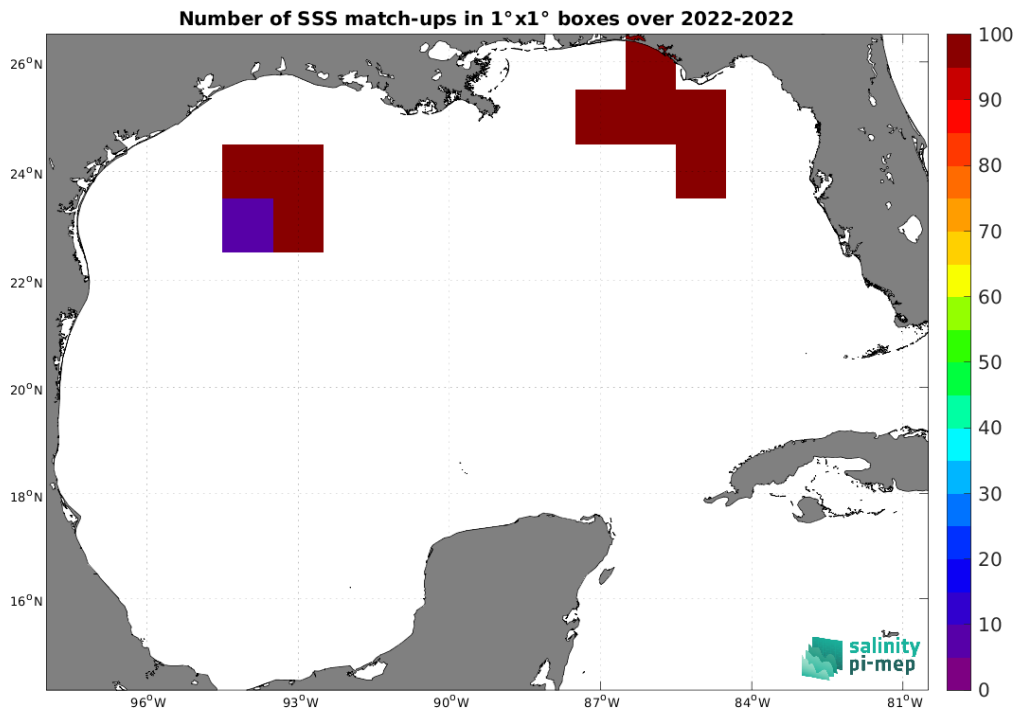
Figure 4: Number of SSS match-ups between Saildrone SSS and the SMAP SSS L3 v5 - Monthly (RSS) SSS product for the Gulf of Mexico Pi-MEP region over 1°×1° boxes and for the full satellite product period.
