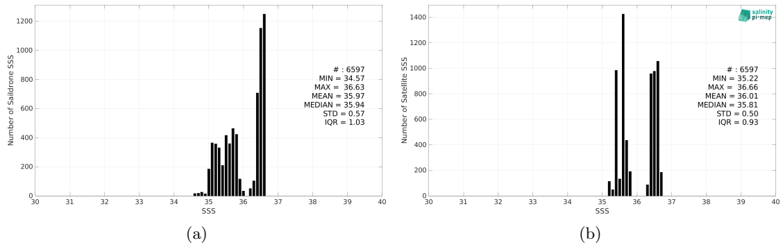
Figure 2: Histograms of SSS from Saildrone (a) and SMAP SSS L3 v5 - Monthly (RSS) (b) considering all match-up pairs per bins of 0.1 over the Gulf of Mexico Pi-MEP region and for the full satellite product period.
