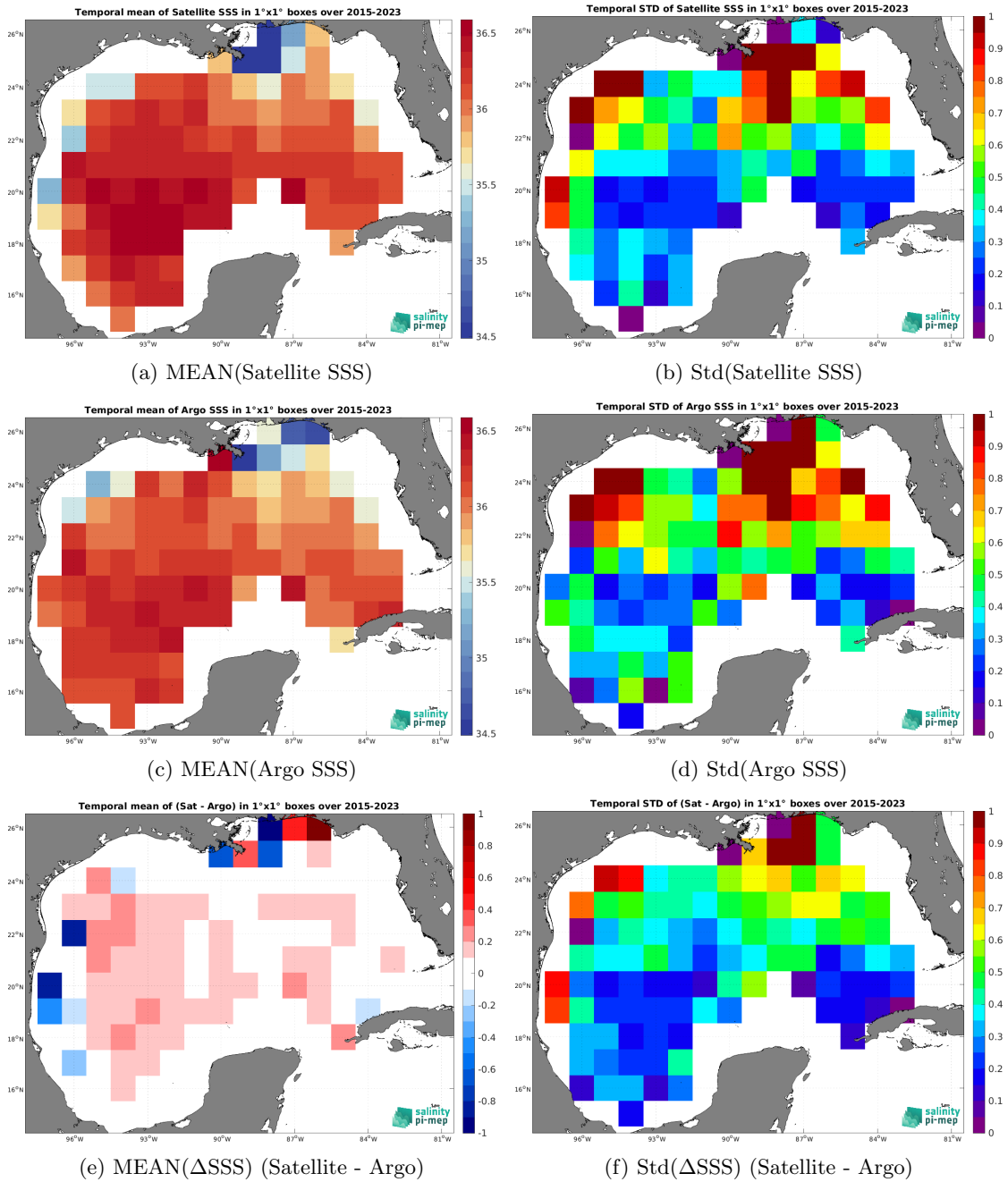
Figure 6: Temporal mean (left) and Std (right) of SSS from SMAP SSS L3 v5 - Monthly (RSS) (top), Argo (middle), and of \Delta SSS (Satellite - Argo). Only match-up pairs are used to generate these maps.
