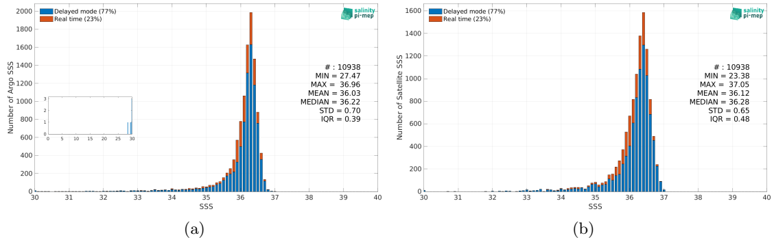
Figure 2: Histograms of SSS from Argo (a) and SMAP SSS L3 v5 - Monthly (RSS) (b) considering all match-up pairs per bins of 0.1 over the Gulf of Mexico Pi-MEP region and for the full satellite product period.
