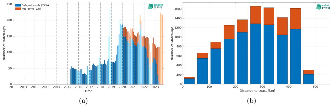
Figure 1: Number of match-ups between Argo and SMAP SSS L3 v5 - Monthly (RSS) SSS as a function of time (a) and as function of the distance to coast (b) over the Gulf of Mexico Pi-MEP region and for the full satellite product period.
