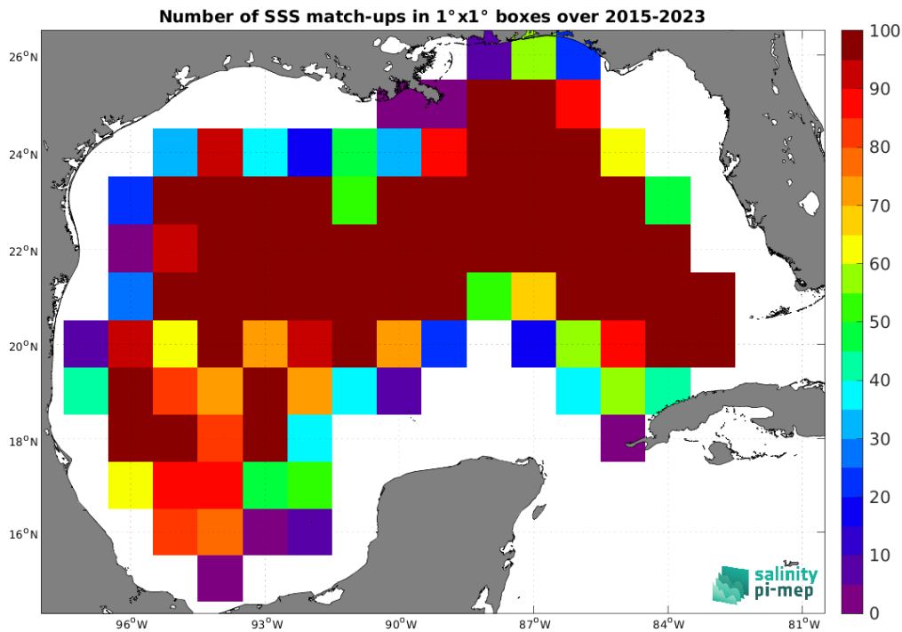
Figure 4: Number of SSS match-ups between Argo SSS and the SMAP SSS L3 v5 - Monthly (RSS) SSS product for the Gulf of Mexico Pi-MEP region over 1^\circ \times 1^\circ boxes and for the full satellite product period.
