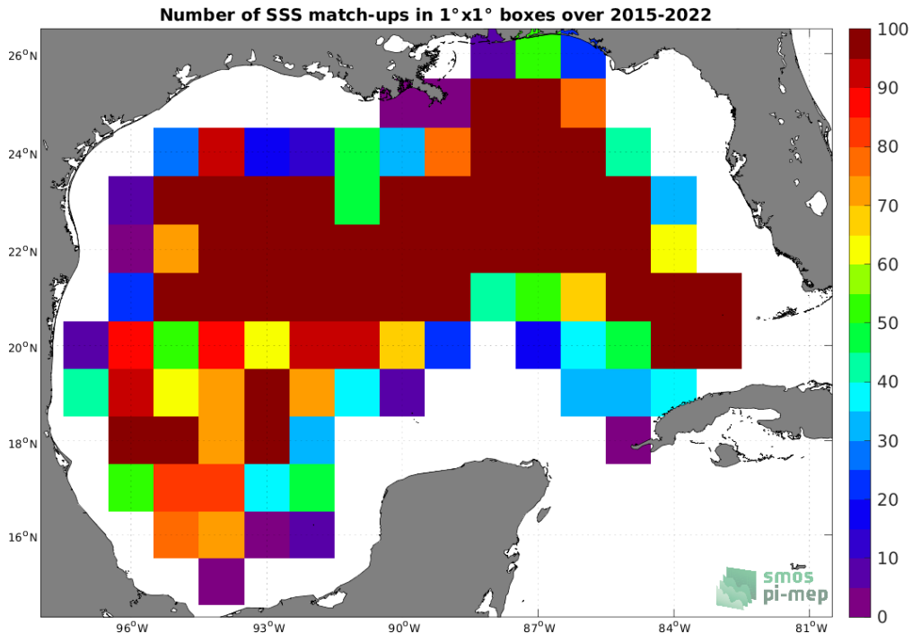
Figure 4: Number of SSS match-ups between Argo SSS and the SMAP SSS L3 v5 - Monthly (RSS) SSS product for the Gulf of Mexico Pi-MEP region over 1°x1° boxes and for the full satellite product period.
