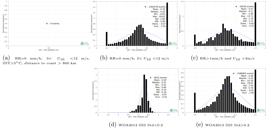
Figure 13: Normalized histogram of \Delta\text{SSS} (SMAP SSS L3 v4 - 8-Day running (RSS) - TSG (SAMOS)) for 5 different subdatasets corresponding to: RR=0 mm/h, 3 < U_{10} < 12 m/s, SST > 5^\circ\text{C} , distance to coast > 800 km (a), RR=0 mm/h, 3 < U_{10} < 12 m/s (b), RR > 1 mm/h and U_{10} < 4 m/s (c), WOA2013 SSS Std < 0.2 (d), WOA2013 SSS Std > 0.2 (e).
