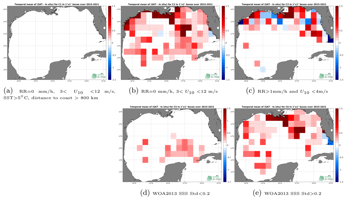
Figure 12: Temporal mean gridded over spatial boxes of size 1^\circ \times 1^\circ of \Delta SSS (SMAP SSS L3 v4 - 8-Day running (RSS) - TSG (SAMOS)) for 5 different subdatasets corresponding to:RR=0 mm/h, 3 < U_{10} < 12 m/s, SST >5^\circ\text{C} , distance to coast > 800 km (a), RR=0 mm/h, 3 < U_{10} < 12 m/s (b), RR >1 mm/h and U_{10} < 4 m/s (c), WOA2013 SSS Std <0.2 (d), WOA2013 SSS Std >0.2 (e).
