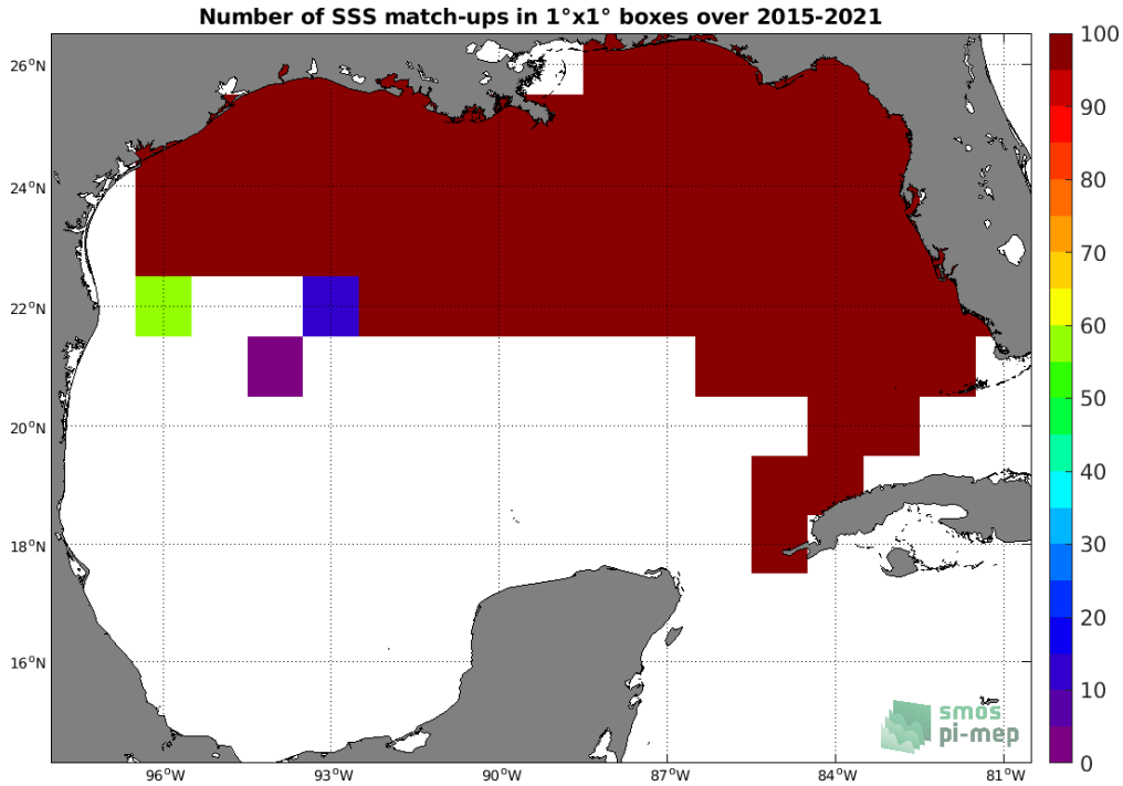
Figure 4: Number of SSS match-ups between TSG (SAMOS) SSS and the SMAP SSS L3 v4 - 8-Day running (RSS) SSS product for the Gulf of Mexico Pi-MEP region over 1^\circ \times 1^\circ boxes and for the full satellite product period.
