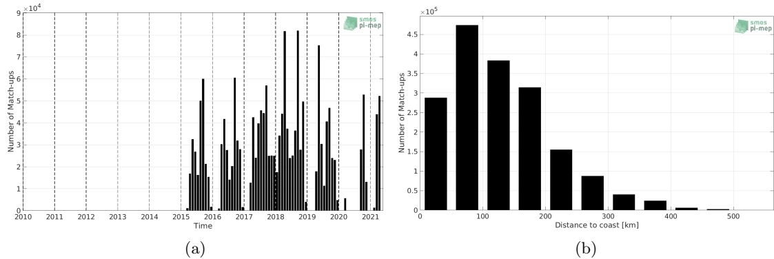
Figure 1: Number of match-ups between TSG (SAMOS) and SMAP SSS L3 v4 - 8-Day running (RSS) SSS as a function of time (a) and as function of the distance to coast (b) over the Gulf of Mexico Pi-MEP region and for the full satellite product period.
