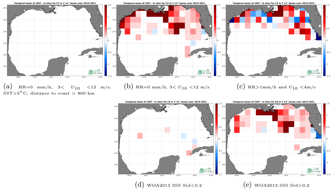
Figure 12: Temporal mean gridded over spatial boxes of size 1^{\circ}\times 1^{\circ} of \Delta\text{SSS} (SMAP SSS L3 v4 - 8-Day running (RSS) - TSG (SAMOS)) for 5 different subdatasets corresponding to:RR=0 mm/h, 3 < U_{10} < 12 m/s, SST > 5^{\circ}\text{C} , distance to coast > 800 km (a), RR=0 mm/h, 3 < U_{10} < 12 m/s (b), RR > 1 mm/h and U_{10} < 4 m/s (c), WOA2013 SSS Std < 0.2 (d), WOA2013 SSS Std > 0.2 (e).
