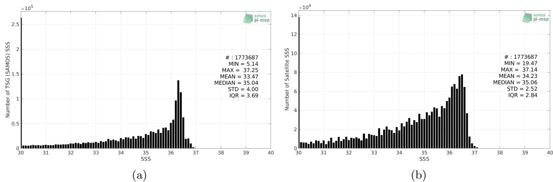
Figure 2: Histograms of SSS from TSG (SAMOS) (a) and SMAP SSS L3 v4 - 8-Day running (RSS) (b) considering all match-up pairs per bins of 0.1 over the Gulf of Mexico Pi-MEP region and for the full satellite product period.
