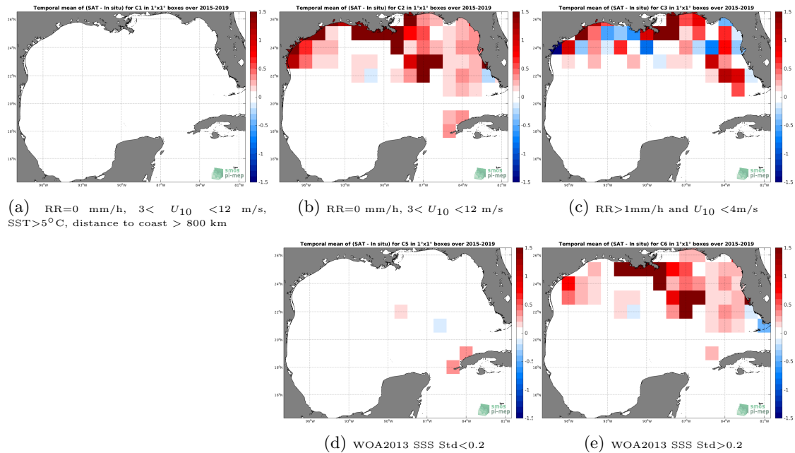
Figure 12: Temporal mean gridded over spatial boxes of size 1^{\circ}\times 1^{\circ} of \Delta\text{SSS} (SMAP-L3-RSS-V4-8DAY-RUNNING - TSG-SAMOS) for 5 different subdatasets corresponding to:RR=0 mm/h, 3 < U_{10} < 12 m/s, SST >5^{\circ}\text{C} , distance to coast > 800 km (a), RR=0 mm/h, 3 < U_{10} < 12 m/s (b), RR >1 mm/h and U_{10} < 4 m/s (c), WOA2013 SSS Std <0.2 (d), WOA2013 SSS Std >0.2 (e).
