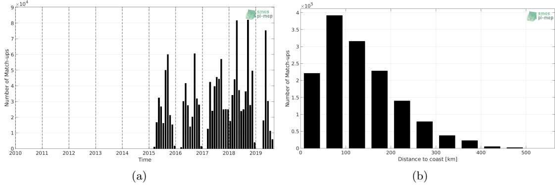
Figure 1: Number of match-ups between TSG-SAMOS and SMAP-L3-RSS-V4-8DAY-RUNNING SSS as a function of time (a) and as function of the distance to coast (b) over the Gulf of Mexico Pi-MEP region and for the full satellite product period.
