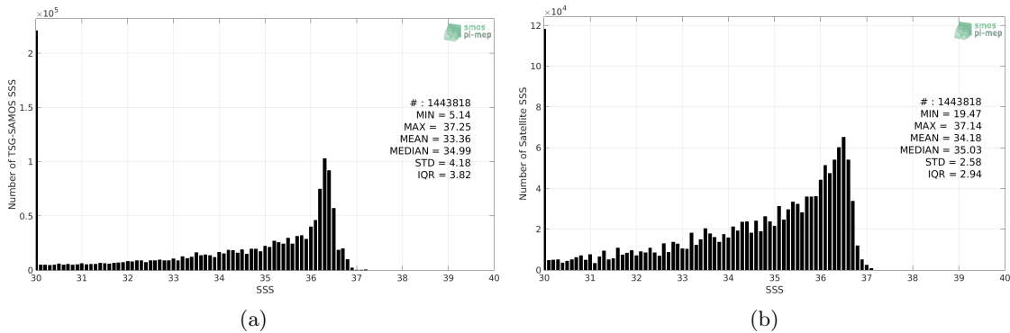
Figure 2: Histograms of SSS from TSG-SAMOS (a) and SMAP-L3-RSS-V4-8DAY-RUNNING (b) considering all match-up pairs per bins of 0.1 over the Gulf of Mexico Pi-MEP region and for the full satellite product period.
