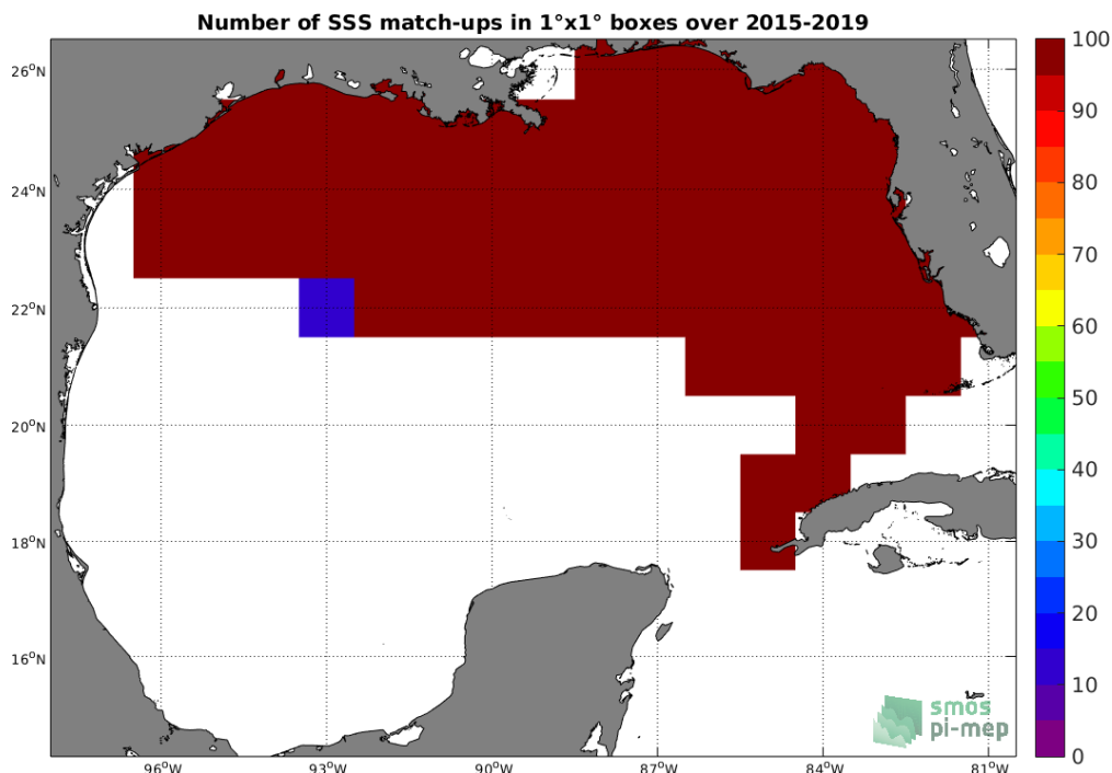
Figure 4: Number of SSS match-ups between TSG-SAMOS SSS and the SMAP-L3-RSS-V4-8DAY-RUNNING SSS product for the Gulf of Mexico Pi-MEP region over 1°x1° boxes and for the full satellite product period.
