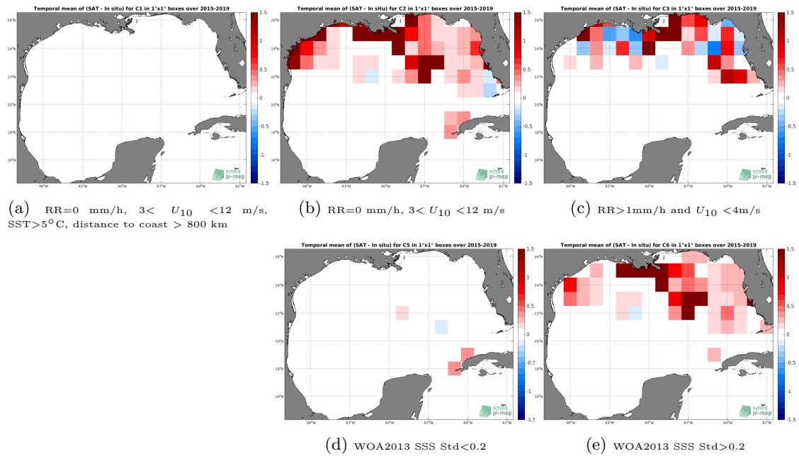
Figure 12: Temporal mean gridded over spatial boxes of size 1^\circ \times 1^\circ of \Delta SSS (SMAP-L3-RSS-V4-8DAY-RUNNING - TSG-SAMOS) for 5 different subdatasets corresponding to:RR=0 mm/h, 3 < U_{10} < 12 m/s, SST >5^\circ C, distance to coast > 800 km (a), RR=0 mm/h, 3 < U_{10} < 12 m/s (b), RR >1 mm/h and U_{10} < 4 m/s (c), WOA2013 SSS Std <0.2 (d), WOA2013 SSS Std >0.2 (e).
