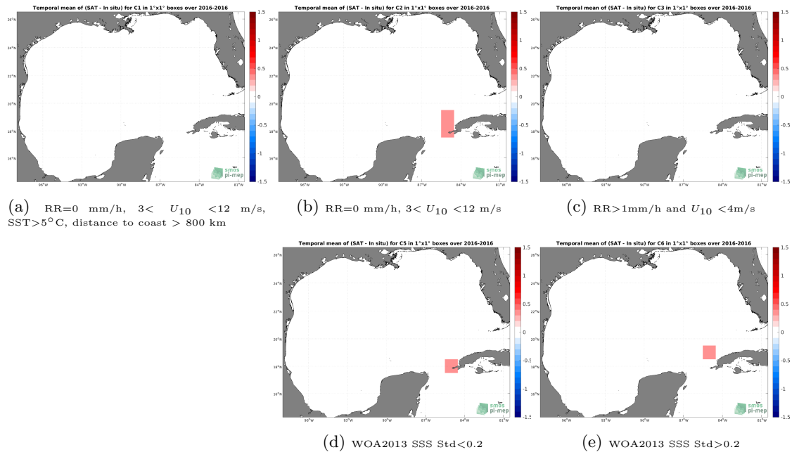
Figure 12: Temporal mean gridded over spatial boxes of size 1^{\circ}\times 1^{\circ} of \Delta\text{SSS} (SMAP SSS L3 v4 - 8-Day running (RSS) - TSG (LEGOS-DM)) for 5 different subdatasets corresponding to:RR=0 mm/h, 3 < U_{10} < 12 m/s, SST >5^{\circ}\text{C} , distance to coast > 800 km (a), RR=0 mm/h, 3 < U_{10} < 12 m/s (b), RR >1 mm/h and U_{10} < 4 m/s (c), WOA2013 SSS Std <0.2 (d), WOA2013 SSS Std >0.2 (e).
