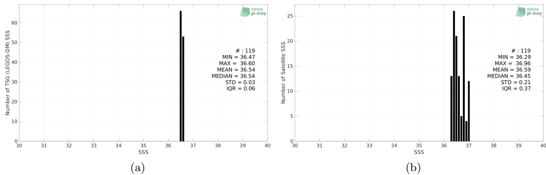
Figure 2: Histograms of SSS from TSG (LEGOS-DM) (a) and SMAP SSS L3 v4 - 8-Day running (RSS) (b) considering all match-up pairs per bins of 0.1 over the Gulf of Mexico Pi-MEP region and for the full satellite product period.
