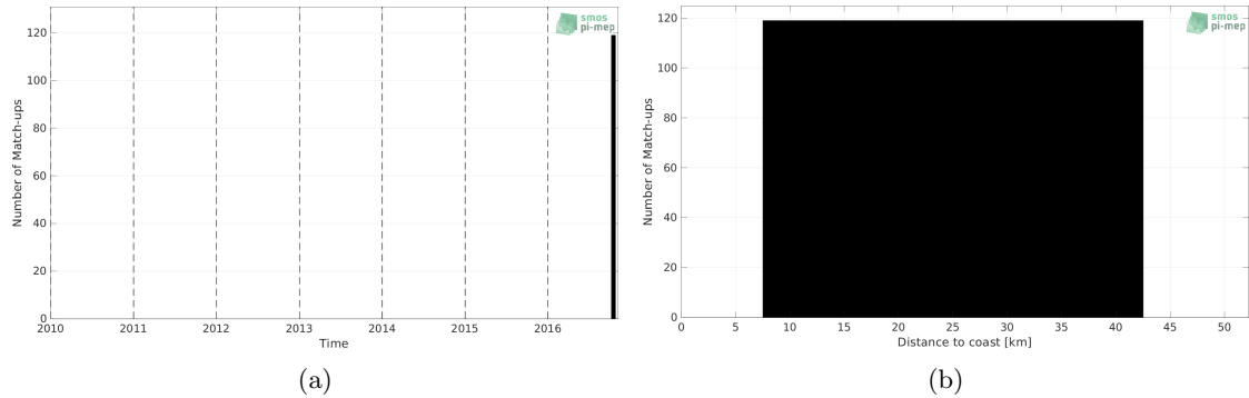
Figure 1: Number of match-ups between TSG (LEGOS-DM) and SMAP SSS L3 v4 - 8-Day running (RSS) SSS as a function of time (a) and as function of the distance to coast (b) over the Gulf of Mexico Pi-MEP region and for the full satellite product period.
