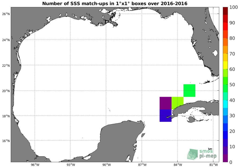
Figure 4: Number of SSS match-ups between TSG (LEGOS-DM) SSS and the SMAP SSS L3 v4 - 8-Day running (RSS) SSS product for the Gulf of Mexico Pi-MEP region over 1°x1° boxes and for the full satellite product period.
