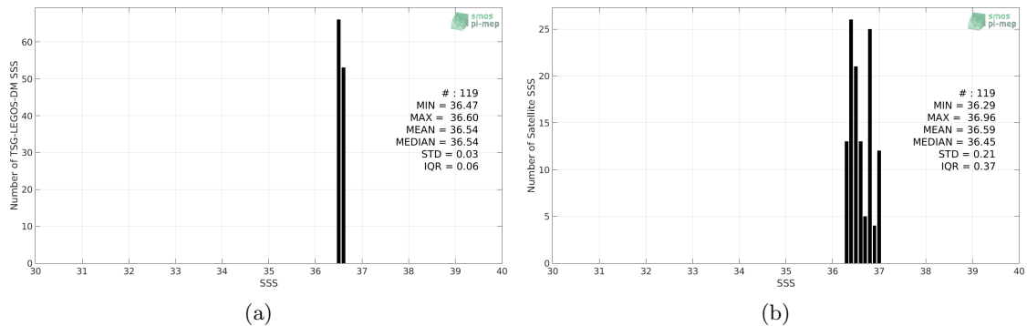
Figure 2: Histograms of SSS from TSG-LEGOS-DM (a) and SMAP-L3-RSS-V4-8DAY-RUNNING (b) considering all match-up pairs per bins of 0.1 over the Gulf of Mexico Pi-MEP region and for the full satellite product period.
