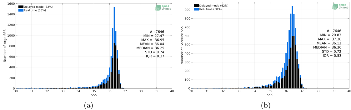
Figure 2: Histograms of SSS from Argo (a) and SMAP SSS L3 v4 - 8-Day running (RSS) (b) considering all match-up pairs per bins of 0.1 over the Gulf of Mexico Pi-MEP region and for the full satellite product period.
