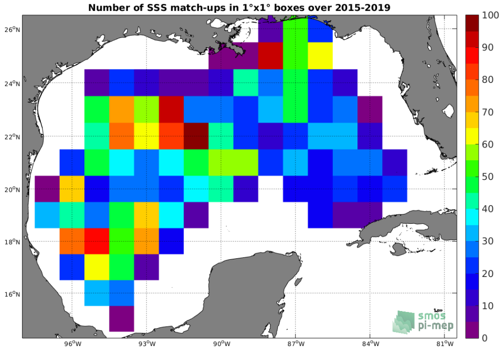
Figure 4: Number of SSS match-ups between Argos SSS and the SMAP-L3-RSS-V4-8DAY-RUNNING SSS product for the Gulf of Mexico Pi-MEP region over 1°x1° boxes and for the full satellite product period.
