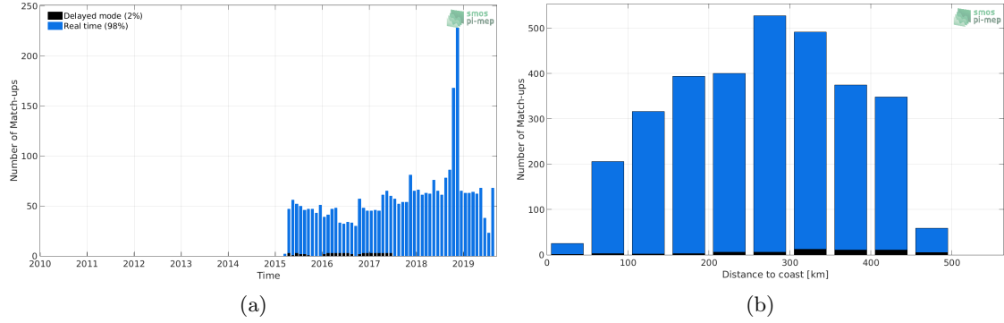
Figure 1: Number of match-ups between Argo and SMAP-L3-RSS-V4-8DAY-RUNNING SSS as a function of time (a) and as function of the distance to coast (b) over the Gulf of Mexico Pi-MEP region and for the full satellite product period.
