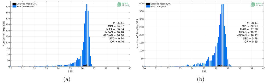
Figure 2: Histograms of SSS from Argo (a) and SMAP-L3-RSS-V4-8DAY-RUNNING (b) considering all match-up pairs per bins of 0.1 over the Gulf of Mexico Pi-MEP region and for the full satellite product period.
