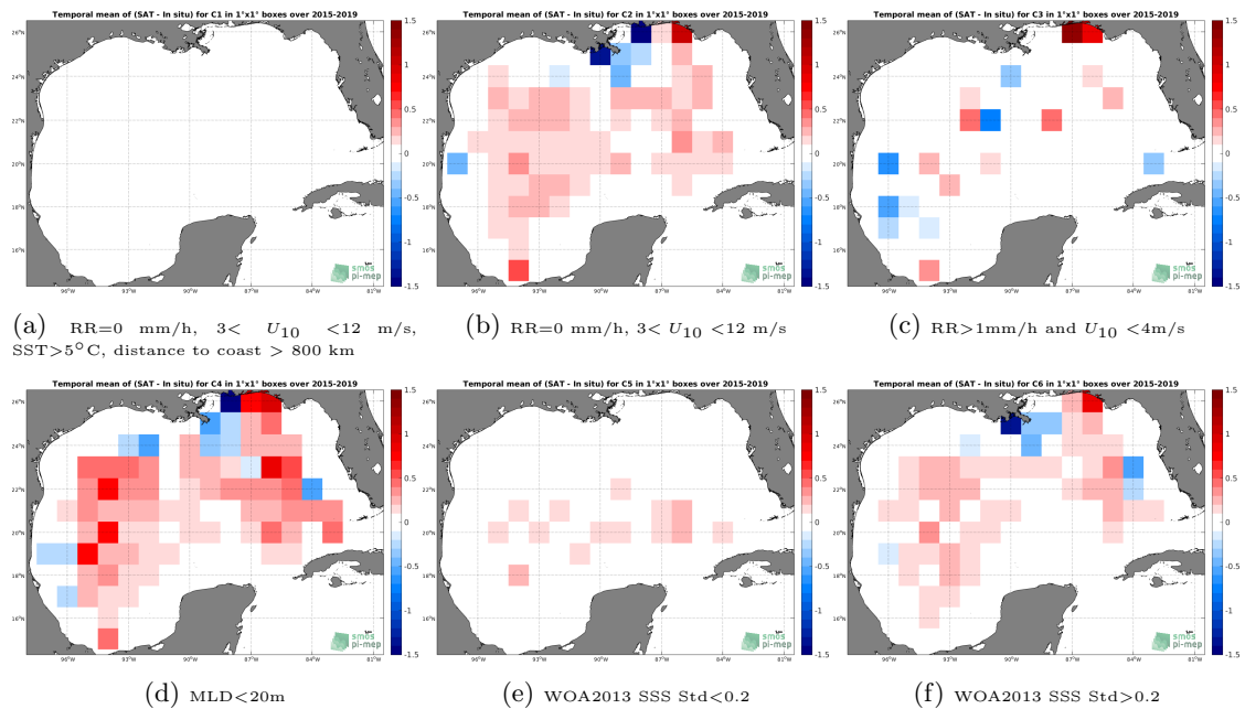
Figure 12: Temporal mean gridded over spatial boxes of size 1^\circ \times 1^\circ of \Delta SSS (SMAP-L3-RSS-V4-8DAY-RUNNING - Argo) for 6 different subdatasets corresponding to:RR=0 mm/h, 3 < U_{10} < 12 m/s, SST >5^\circ C, distance to coast > 800 km (a), RR=0 mm/h, 3 < U_{10} < 12 m/s (b), RR >1 mm/h and U_{10} < 4 m/s (c),MLD <20 m (d),WOA2013 SSS Std <0.2 (e),WOA2013 SSS Std >0.2 (f).
