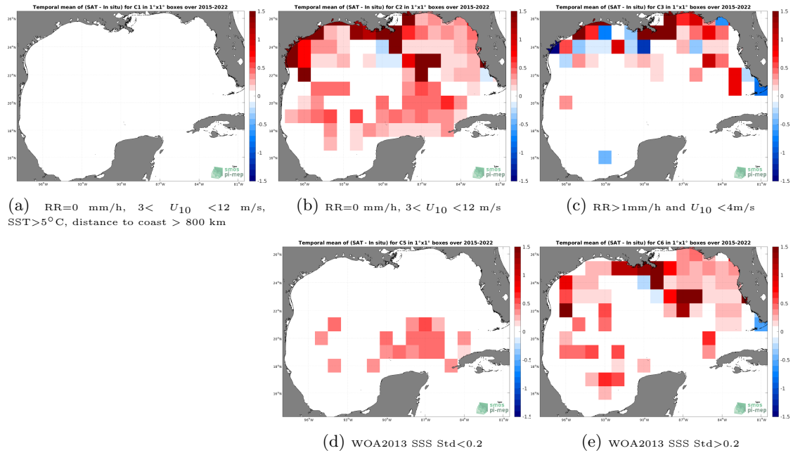
Figure 12: Temporal mean gridded over spatial boxes of size 1^\circ \times 1^\circ of \Delta SSS (SMAP SSS L3 v4 - Monthly (RSS) - TSG (SAMOS)) for 5 different subdatasets corresponding to:RR=0 mm/h, 3 < U_{10} < 12 m/s, SST >5^\circ\text{C} , distance to coast > 800 km (a), RR=0 mm/h, 3 < U_{10} < 12 m/s (b), RR >1 mm/h and U_{10} < 4 m/s (c), WOA2013 SSS Std <0.2 (d), WOA2013 SSS Std >0.2 (e).
