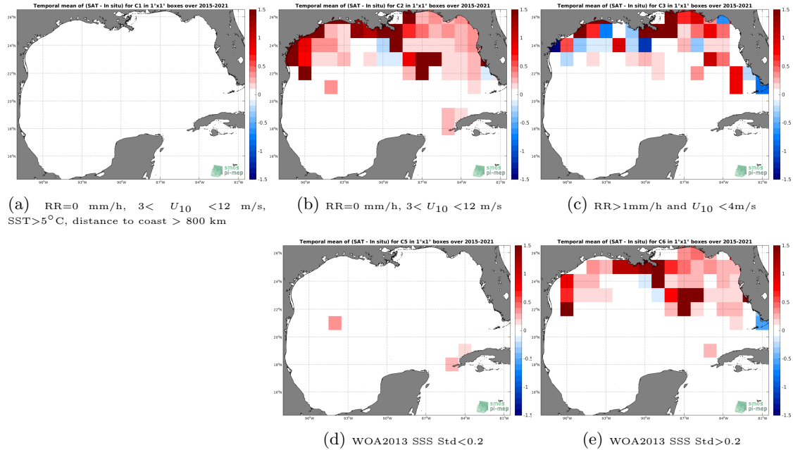
Figure 12: Temporal mean gridded over spatial boxes of size 1^{\circ}\times 1^{\circ} of \Delta\text{SSS} (SMAP SSS L3 v4 - Monthly (RSS) - TSG (SAMOS)) for 5 different subdatasets corresponding to:RR=0 mm/h, 3 < U_{10} < 12 m/s, SST >5^{\circ}\text{C} , distance to coast > 800 km (a), RR=0 mm/h, 3 < U_{10} < 12 m/s (b), RR >1 mm/h and U_{10} < 4 m/s (c), WOA2013 SSS Std <0.2 (d), WOA2013 SSS Std >0.2 (e).
