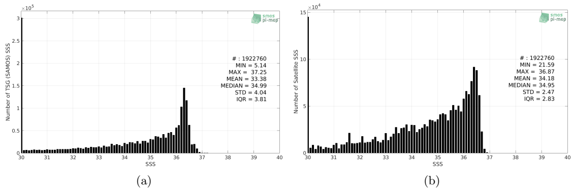
Figure 2: Histograms of SSS from TSG (SAMOS) (a) and SMAP SSS L3 v4 - Monthly (RSS) (b) considering all match-up pairs per bins of 0.1 over the Gulf of Mexico Pi-MEP region and for the full satellite product period.
