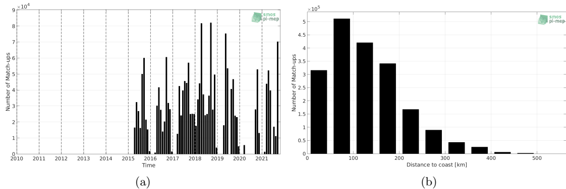
Figure 1: Number of match-ups between TSG (SAMOS) and SMAP SSS L3 v4 - Monthly (RSS) SSS as a function of time (a) and as function of the distance to coast (b) over the Gulf of Mexico Pi-MEP region and for the full satellite product period.
