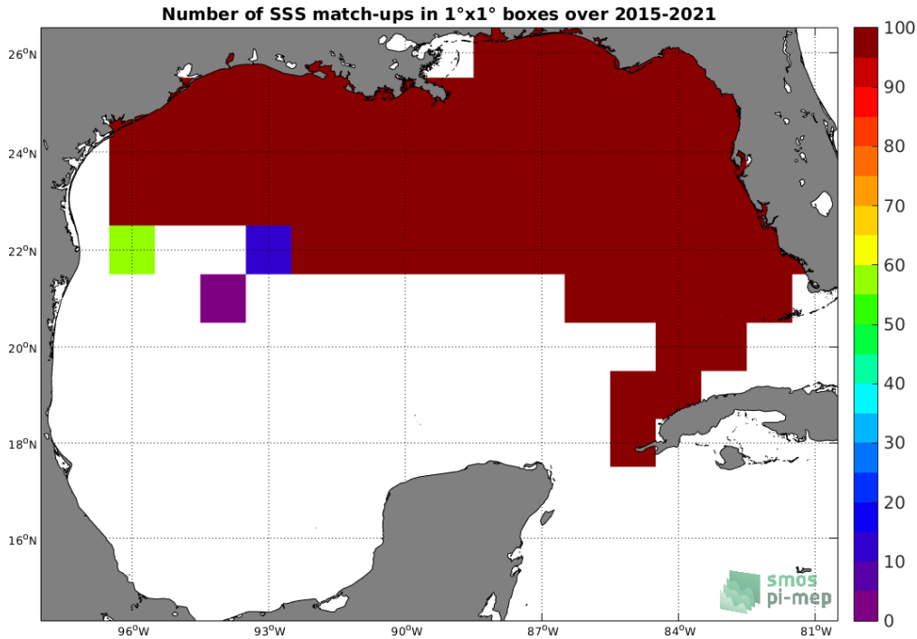
Figure 4: Number of SSS match-ups between TSG (SAMOS) SSS and the SMAP SSS L3 v4 - Monthly (RSS) SSS product for the Gulf of Mexico Pi-MEP region over 1^\circ \times 1^\circ boxes and for the full satellite product period.
