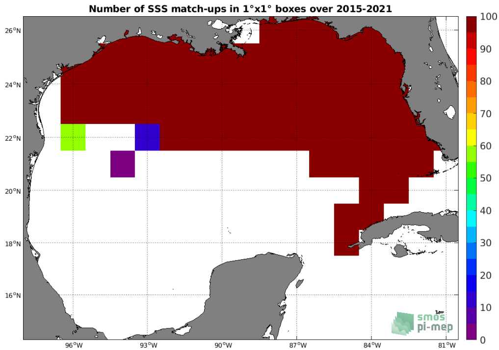
Figure 4: Number of SSS match-ups between TSG (SAMOS) SSS and the SMAP SSS L3 v4 - Monthly (RSS) SSS product for the Gulf of Mexico Pi-MEP region over 1°x1° boxes and for the full satellite product period.
