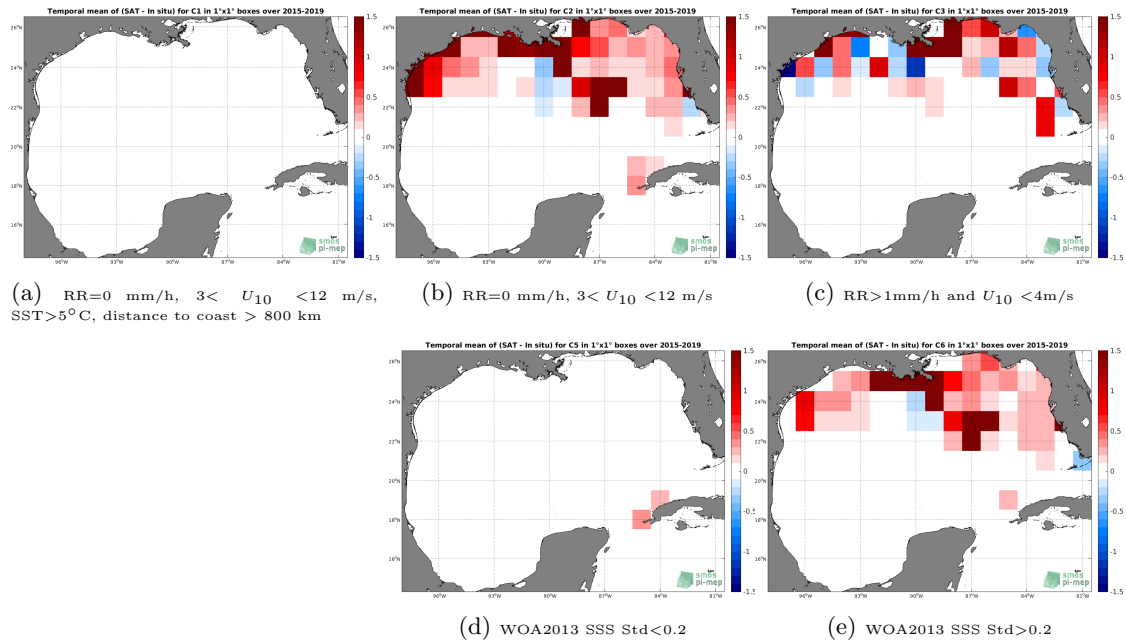
Figure 12: Temporal mean gridded over spatial boxes of size 1^{\circ}\times 1^{\circ} of \Delta\text{SSS} (SMAP-L3-RSS-V4-MONTHLY - TSG-SAMOS) for 5 different subdatasets corresponding to:RR=0 mm/h, 3 < U_{10} < 12 m/s, SST >5^{\circ}\text{C} , distance to coast > 800 km (a), RR=0 mm/h, 3 < U_{10} < 12 m/s (b), RR >1 mm/h and U_{10} < 4 m/s (c), WOA2013 SSS Std <0.2 (d), WOA2013 SSS Std >0.2 (e).
