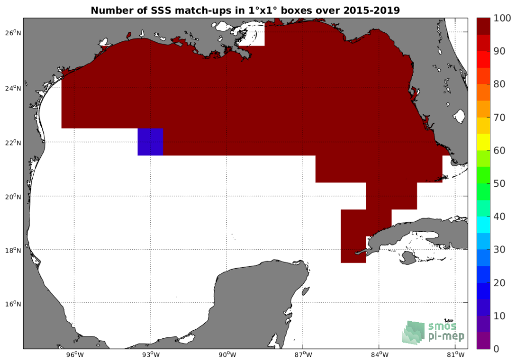
Figure 4: Number of SSS match-ups between TSG-SAMOS SSS and the SMAP-L3-RSS-V4-MONTHLY SSS product for the Gulf of Mexico Pi-MEP region over 1°x1° boxes and for the full satellite product period.
