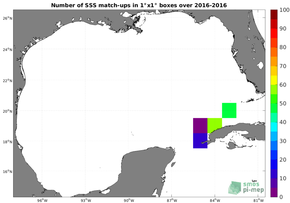
Figure 4: Number of SSS match-ups between TSG (LEGOS-DM) SSS and the SMAP SSS L3 v4 - Monthly (RSS) SSS product for the Gulf of Mexico Pi-MEP region over 1^\circ \times 1^\circ boxes and for the full satellite product period.
