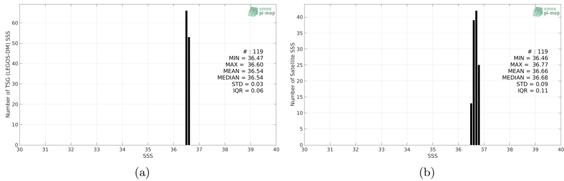
Figure 2: Histograms of SSS from TSG (LEGOS-DM) (a) and SMAP SSS L3 v4 - Monthly (RSS) (b) considering all match-up pairs per bins of 0.1 over the Gulf of Mexico Pi-MEP region and for the full satellite product period.
