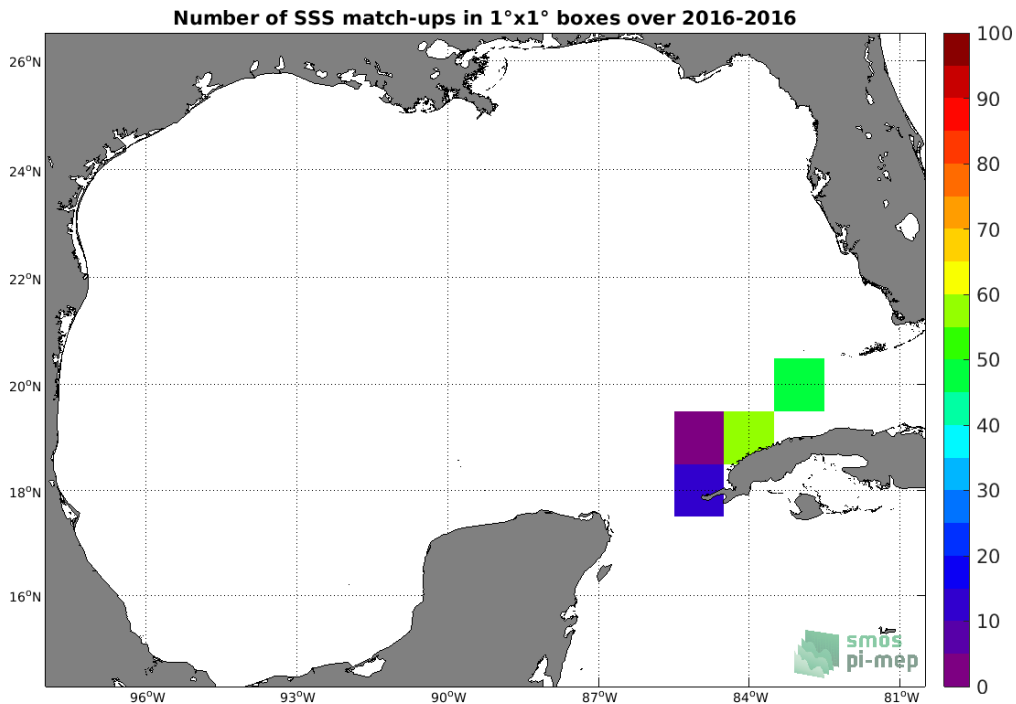
Figure 4: Number of SSS match-ups between TSG (LEGOS-DM) SSS and the SMAP SSS L3 v4 - Monthly (RSS) SSS product for the Gulf of Mexico Pi-MEP region over 1°x1° boxes and for the full satellite product period.
