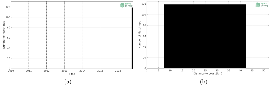
Figure 1: Number of match-ups between TSG (LEGOS-DM) and SMAP SSS L3 v4 - Monthly (RSS) SSS as a function of time (a) and as function of the distance to coast (b) over the Gulf of Mexico Pi-MEP region and for the full satellite product period.
