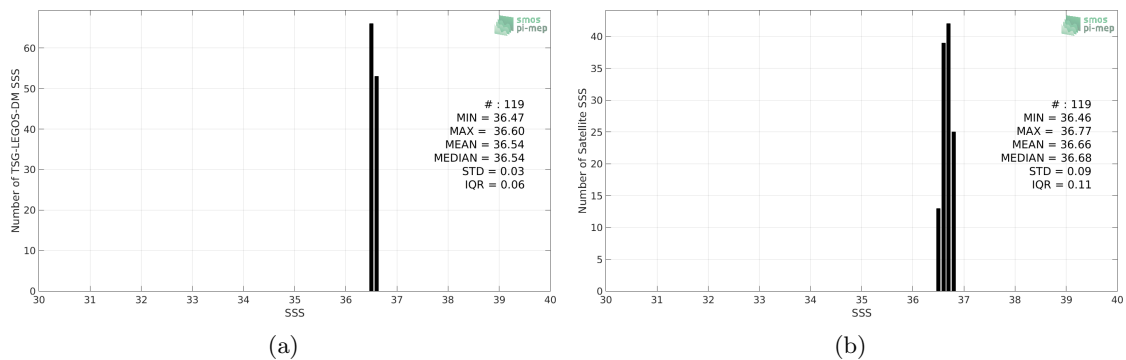
Figure 2: Histograms of SSS from TSG-LEGOS-DM (a) and SMAP-L3-RSS-V4-MONTHLY (b) considering all match-up pairs per bins of 0.1 over the Gulf of Mexico Pi-MEP region and for the full satellite product period.
