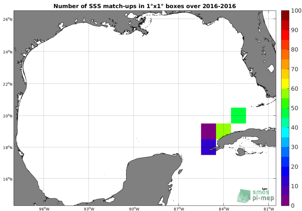
Figure 4: Number of SSS match-ups between TSG-LEGOS-DM SSS and the SMAP-L3-RSS-V4-MONTHLY SSS product for the Gulf of Mexico Pi-MEP region over 1°x1° boxes and for the full satellite product period.
