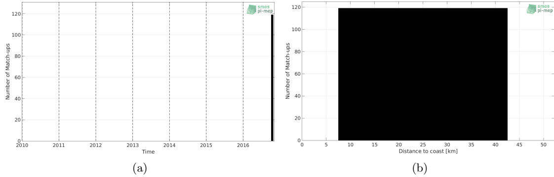
Figure 1: Number of match-ups between TSG-LEGOS-DM and SMAP-L3-RSS-V4-MONTHLY SSS as a function of time (a) and as function of the distance to coast (b) over the Gulf of Mexico Pi-MEP region and for the full satellite product period.
