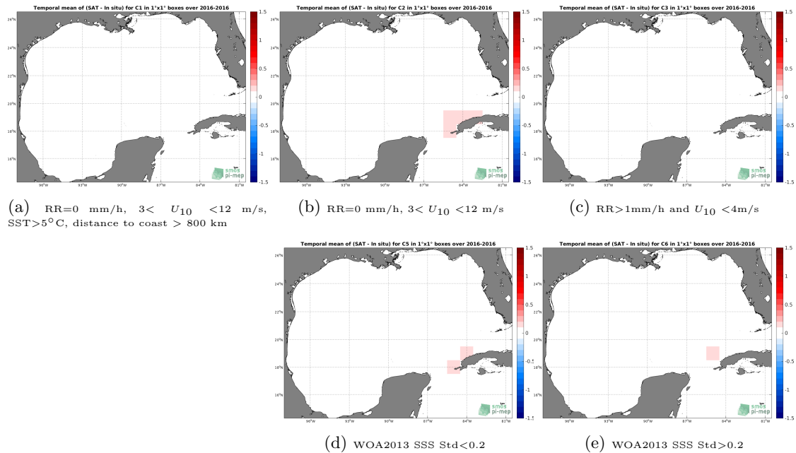
Figure 12: Temporal mean gridded over spatial boxes of size 1^{\circ}\times 1^{\circ} of \Delta\text{SSS} (SMAP-L3-RSS-V4-MONTHLY - TSG-LEGOS-DM) for 5 different subdatasets corresponding to:RR=0 mm/h, 3 < U_{10} < 12 m/s, SST >5^{\circ}\text{C} , distance to coast > 800 km (a), RR=0 mm/h, 3 < U_{10} < 12 m/s (b), RR >1 mm/h and U_{10} < 4 m/s (c), WOA2013 SSS Std <0.2 (d), WOA2013 SSS Std >0.2 (e).
