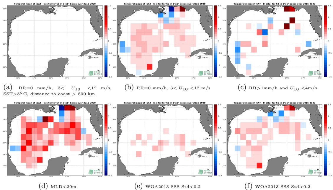
Figure 12: Temporal mean gridded over spatial boxes of size 1^\circ \times 1^\circ of \Delta SSS (SMAP-L3-RSS-V4-MONTHLY - Argo) for 6 different subdatasets corresponding to:RR=0 mm/h, 3 < U_{10} < 12 m/s, SST > 5^\circ C, distance to coast > 800 km (a), RR=0 mm/h, 3 < U_{10} < 12 m/s (b), RR > 1 mm/h and U_{10} < 4 m/s (c),MLD < 20 m (d),WOA2013 SSS Std < 0.2 (e),WOA2013 SSS Std > 0.2 (f).
