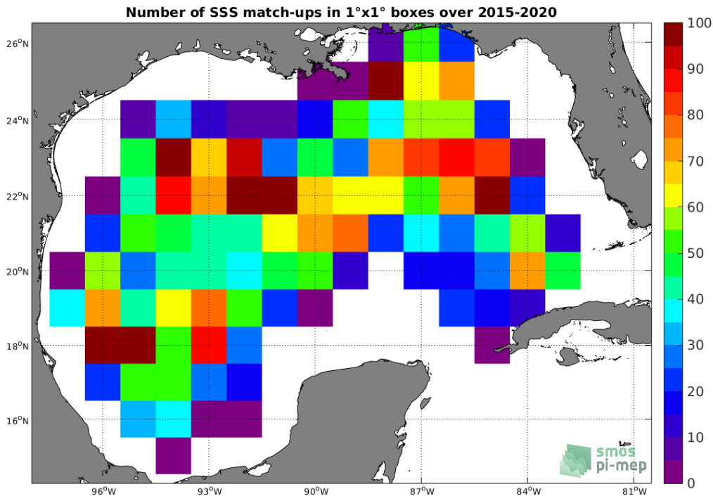
Figure 4: Number of SSS match-ups between Argo SSS and the SMAP-L3-RSS-V4-MONTHLY SSS product for the Gulf of Mexico Pi-MEP region over 1^\circ \times 1^\circ boxes and for the full satellite product period.
