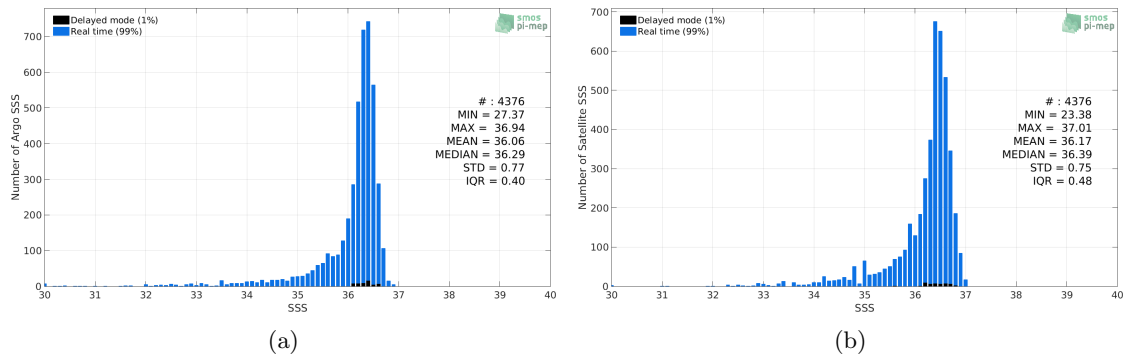
Figure 2: Histograms of SSS from Argo (a) and SMAP-L3-RSS-V4-MONTHLY (b) considering all match-up pairs per bins of 0.1 over the Gulf of Mexico Pi-MEP region and for the full satellite product period.
