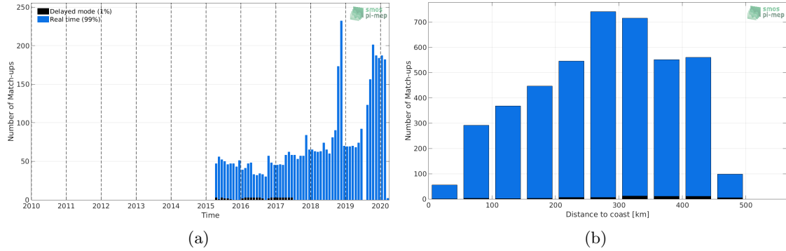
Figure 1: Number of match-ups between Argo and SMAP-L3-RSS-V4-MONTHLY SSS as a function of time (a) and as function of the distance to coast (b) over the Gulf of Mexico Pi-MEP region and for the full satellite product period.
