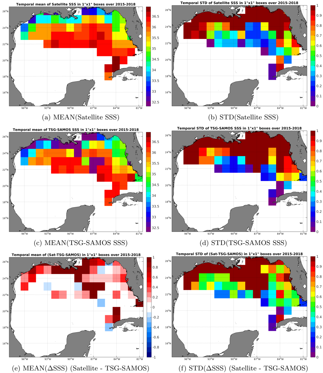
Figure 6: Temporal mean (left) and STD (right) of SSS from SMAP-L3-RSS-V2-8DAY-RUNNING-40KM (top), TSG-SAMOS (middle), and of \Delta SSS (Satellite - TSG-SAMOS). Only match-up pairs are used to generate these maps.
