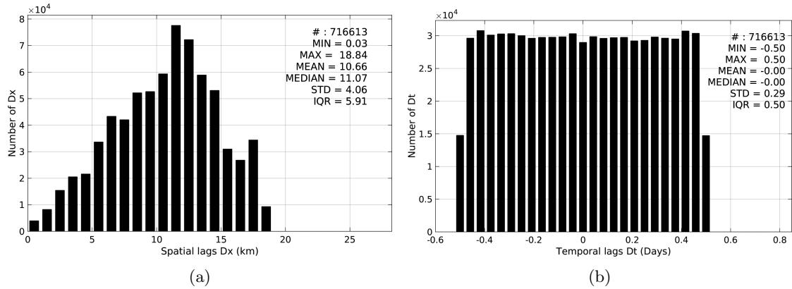
Figure 5: Histograms of the spatial (a) and temporal (b) lags between the time of the TSG-SAMOS measurements and the date of the corresponding SMAP-L3-RSS-V2-8DAY-RUNNING-40KM SSS product.
