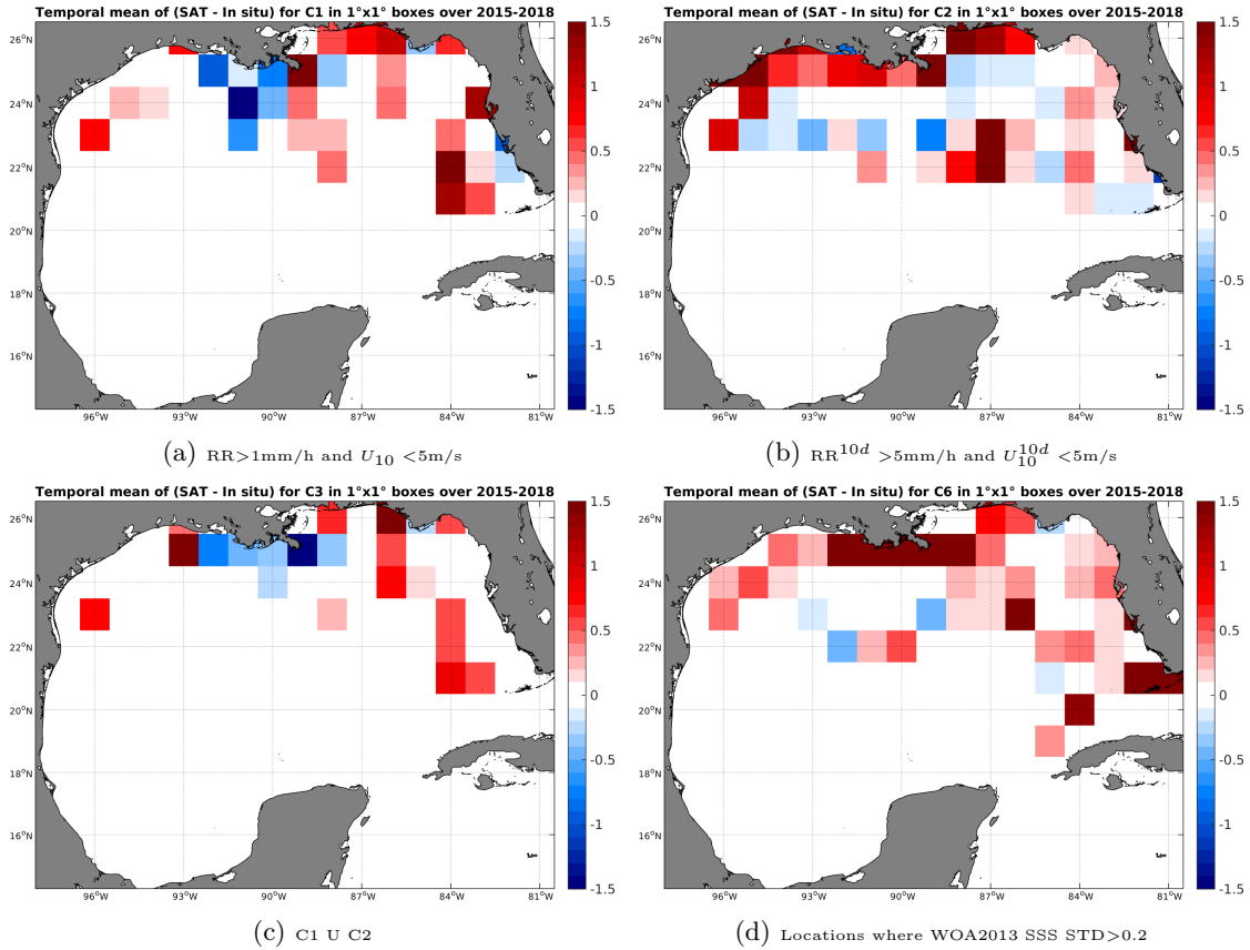
Figure 12: Temporal mean gridded over spatial boxes of size 1^\circ \times 1^\circ of \Delta SSS (SMAP-L3-RSS-V2-8DAY-RUNNING-40KM - TSG-SAMOS) for 4 different subdatasets corresponding to: RR > 1mm/h and U_{10} < 5\text{m/s} (a), RR^{10d} > 5\text{mm/h} and U_{10}^{10d} < 5\text{m/s} (b), C1 U C2 (c), Locations where WOA2013 SSS STD > 0.2 (d).
