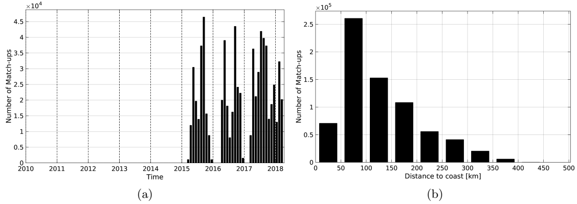
Figure 1: Number of match-ups between TSG-SAMOS and SMAP-L3-RSS-V2-8DAY-RUNNING-40KM SSS as a function of time (a) and as function of the distance to coast (b) over the Gulf of Mexico Pi-MEP region and for the full satellite product period.
