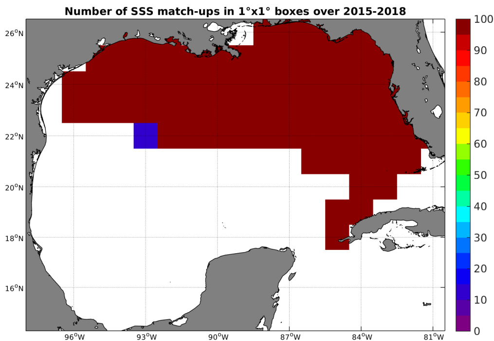
Figure 4: Number of SSS match-ups between TSG-SAMOS SSS and the SMAP-L3-RSS-V2-8DAY-RUNNING-40KM SSS product for the Gulf of Mexico Pi-MEP region over 1^\circ \times 1^\circ boxes and for the full satellite product period.
