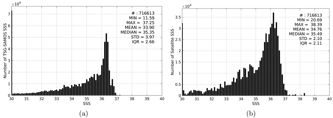
Figure 2: Histograms of SSS from TSG-SAMOS (a) and SMAP-L3-RSS-V2-8DAY-RUNNING-40KM (b) considering all match-up pairs per bins of 0.1 over the Gulf of Mexico Pi-MEP region and for the full satellite product period.
