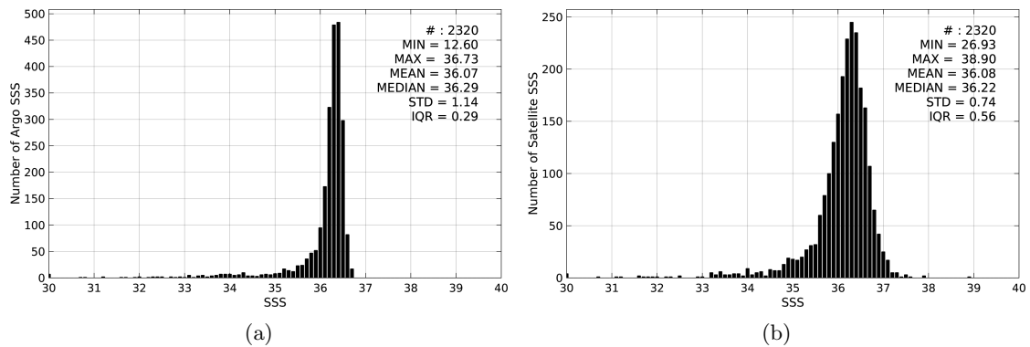
Figure 2: Histograms of SSS from Argo (a) and SMAP-L3-RSS-V2-8DAY-RUNNING-40KM (b) considering all match-up pairs per bins of 0.1 over the Gulf of Mexico Pi-MEP region and for the full satellite product period.
