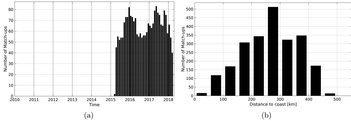
Figure 1: Number of match-ups between Argo and SMAP-L3-RSS-V2-8DAY-RUNNING-40KM SSS as a function of time (a) and as function of the distance to coast (b) over the Gulf of Mexico Pi-MEP region and for the full satellite product period.
