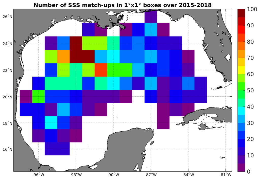
Figure 4: Number of SSS match-ups between Argo SSS and the SMAP-L3-RSS-V2-8DAY-RUNNING-40KM SSS product for the Gulf of Mexico Pi-MEP region over 1^\circ \times 1^\circ boxes and for the full satellite product period.
