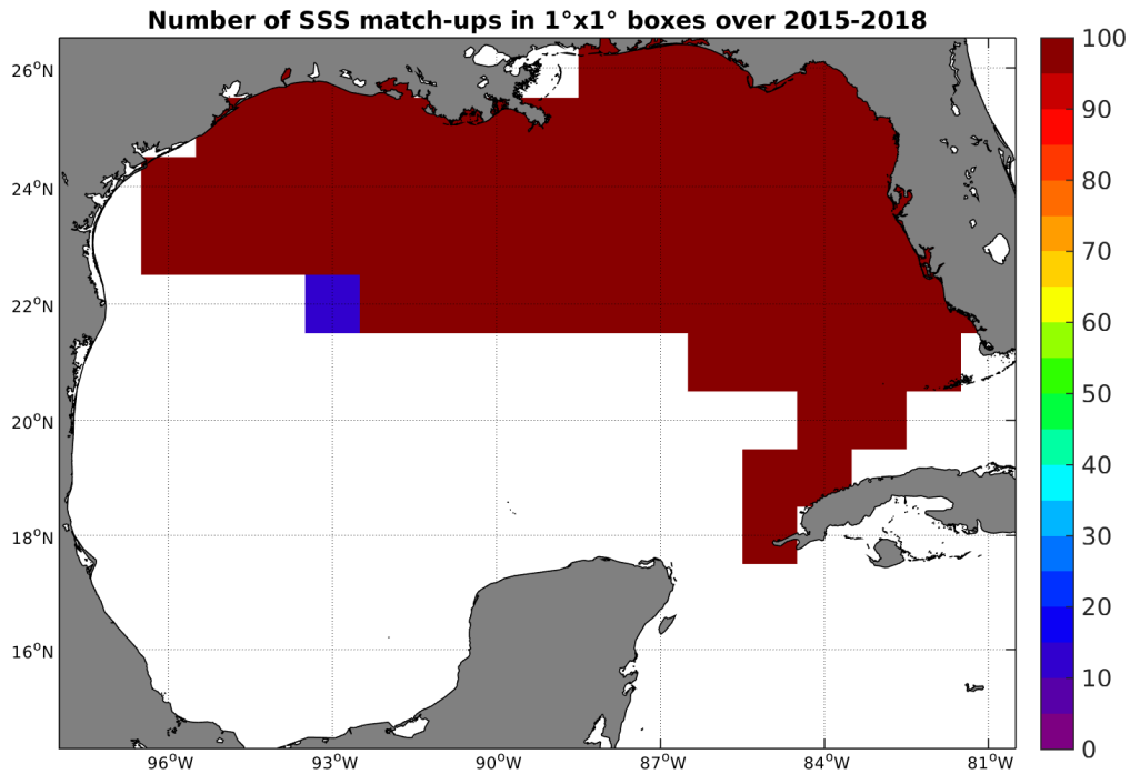
Figure 4: Number of SSS match-ups between TSG-SAMOS SSS and the SMAP-L3-RSS-V2-MONTHLY-0.25DEG-40KM SSS product for the Gulf of Mexico Pi-MEP region over 1^\circ \times 1^\circ boxes and for the full satellite product period.
