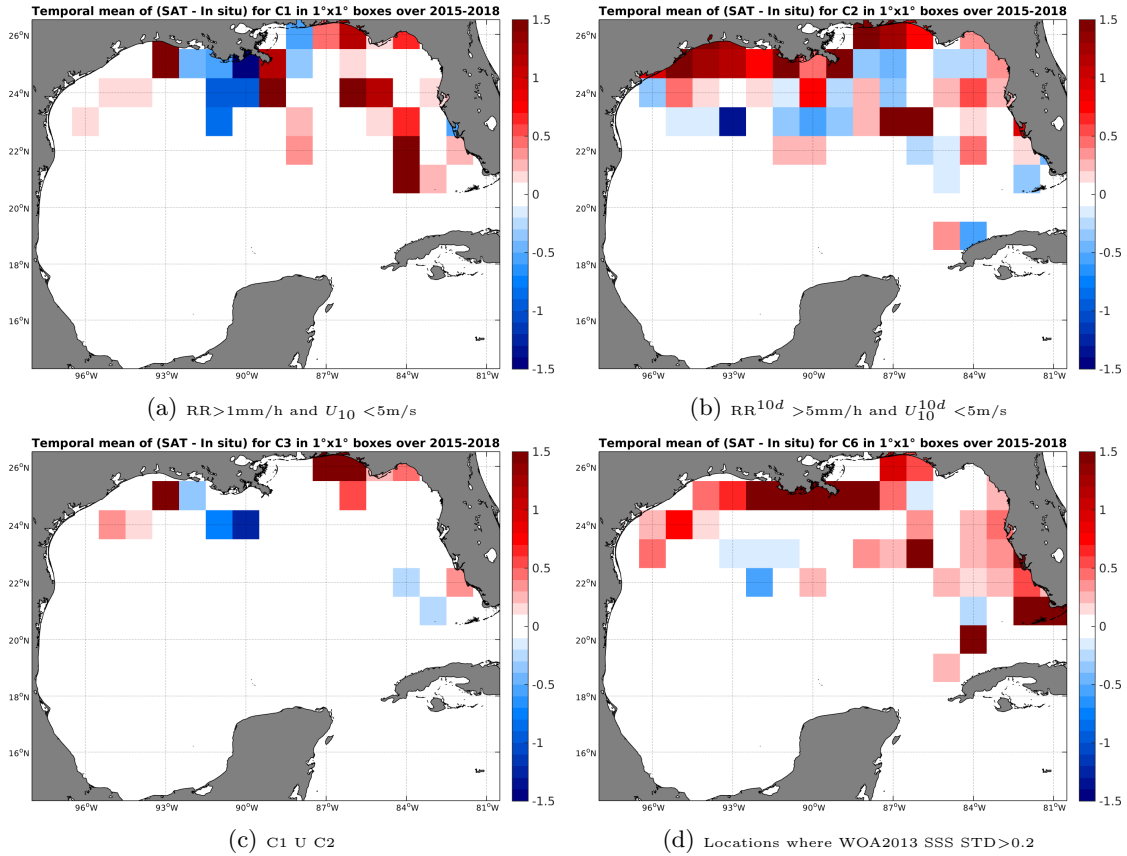
Figure 12: Temporal mean gridded over spatial boxes of size 1^\circ \times 1^\circ of \Delta SSS (SMAP-L3-RSS-V2-MONTHLY-0.25DEG-40KM - TSG-SAMOS) for 4 different subdatasets corresponding to: RR > 1\text{mm/h} and U_{10} < 5\text{m/s} (a), RR^{10d} > 5\text{mm/h} and U_{10}^{10d} < 5\text{m/s} (b), C1 U C2 (c), Locations where WOA2013 SSS STD > 0.2 (d).
