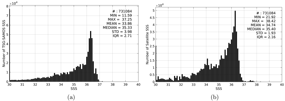
Figure 2: Histograms of SSS from TSG-SAMOS (a) and SMAP-L3-RSS-V2-MONTHLY-0.25DEG-40KM (b) considering all match-up pairs per bins of 0.1 over the Gulf of Mexico Pi-MEP region and for the full satellite product period.
