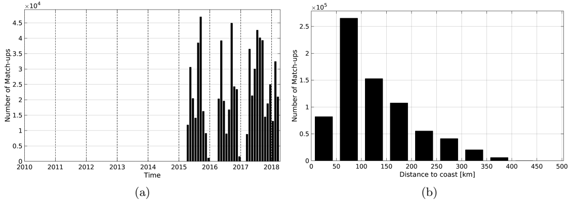
Figure 1: Number of match-ups between TSG-SAMOS and SMAP-L3-RSS-V2-MONTHLY-0.25DEG-40KM SSS as a function of time (a) and as function of the distance to coast (b) over the Gulf of Mexico Pi-MEP region and for the full satellite product period.
