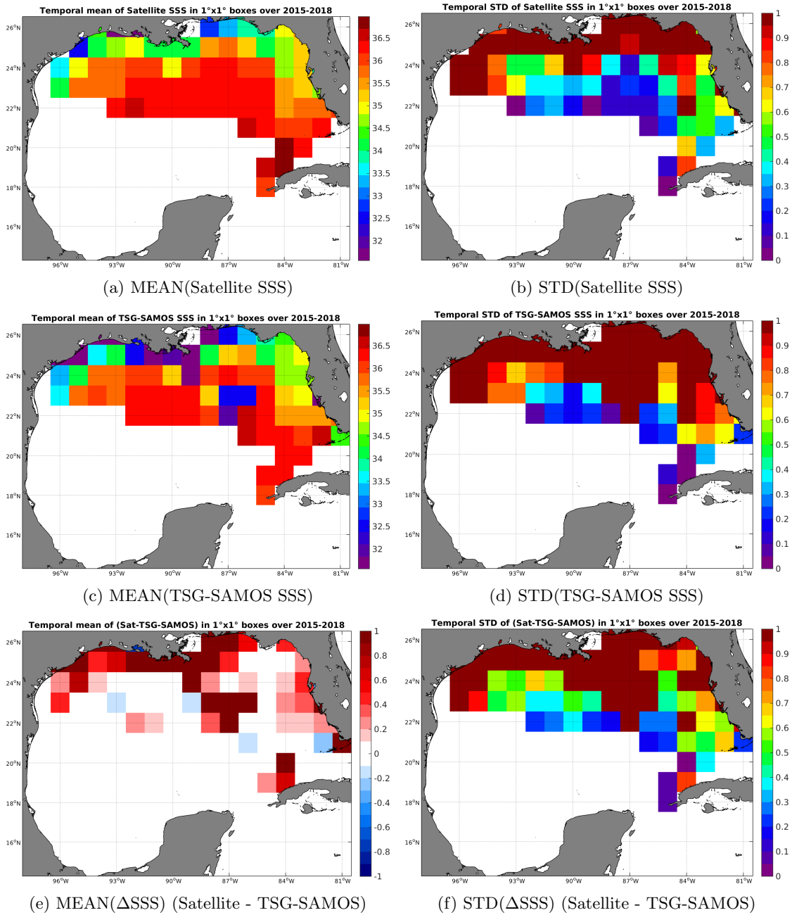
Figure 6: Temporal mean (left) and STD (right) of SSS from SMAP-L3-RSS-V2-MONTHLY-0.25DEG-40KM (top), TSG-SAMOS (middle), and of \Delta SSS (Satellite - TSG-SAMOS). Only match-up pairs are used to generate these maps.
