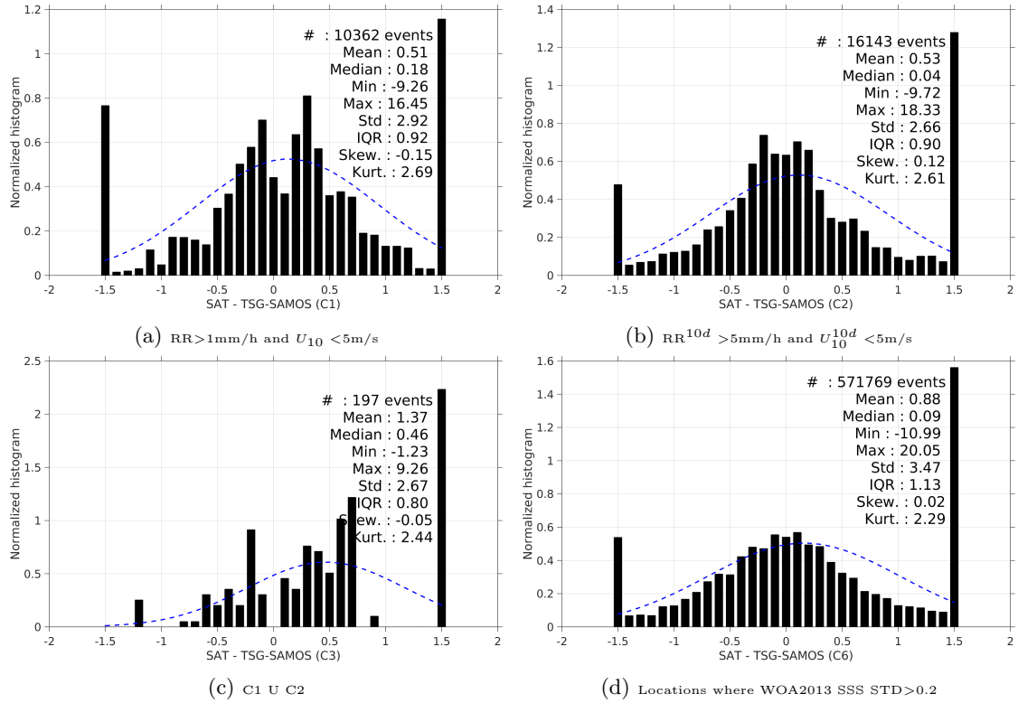
Figure 13: Normalized histogram of \Delta\text{SSS} (SMAP-L3-RSS-V2-MONTHLY-0.25DEG-40KM - TSG-SAMOS) for 6 different subdatasets corresponding to: RR > 1mm/h and U_{10} < 5\text{m/s} (a), RR^{10d} > 5\text{mm/h} and U_{10}^{10d} < 5\text{m/s} (b), C1 U C2 (c), Locations where WOA2013 SSS STD > 0.2 (d).
