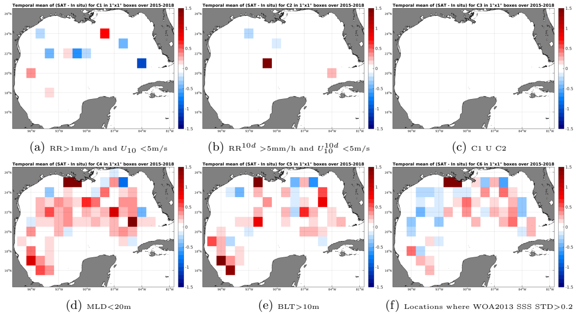
Figure 12: Temporal mean gridded over spatial boxes of size 1^\circ \times 1^\circ of \Delta SSS (SMAP-L3-RSS-V2-MONTHLY-0.25DEG-40KM - Argo) for 6 different subdatasets corresponding to: RR > 1\text{mm/h} and U_{10} < 5\text{m/s} (a), RR^{10d} > 5\text{mm/h} and U_{10}^{10d} < 5\text{m/s} (b), C1 U C2 (c), MLD < 20\text{m} (d), BLT > 10\text{m} (e), Locations where WOA2013 SSS STD > 0.2 (f).
