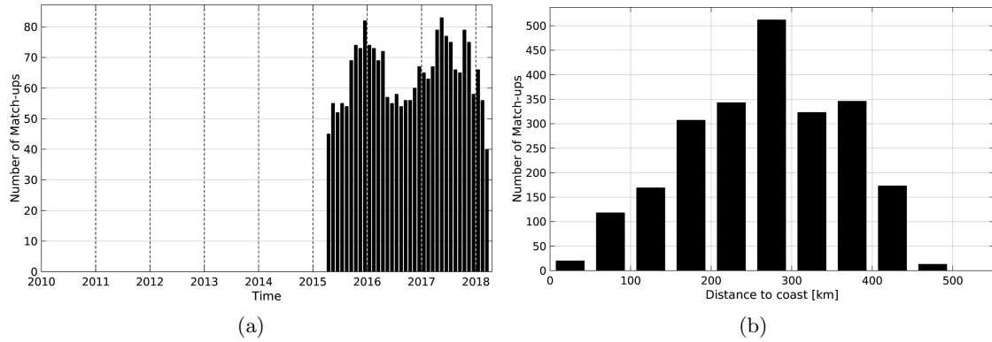
Figure 1: Number of match-ups between Argo and SMAP-L3-RSS-V2-MONTHLY-0.25DEG-40KM SSS as a function of time (a) and as function of the distance to coast (b) over the Gulf of Mexico Pi-MEP region and for the full satellite product period.
