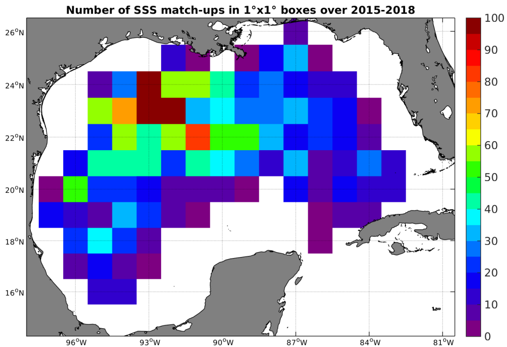
Figure 4: Number of SSS match-ups between Argo SSS and the SMAP-L3-RSS-V2-MONTHLY-0.25DEG-40KM SSS product for the Gulf of Mexico Pi-MEP region over 1°x1° boxes and for the full satellite product period.
