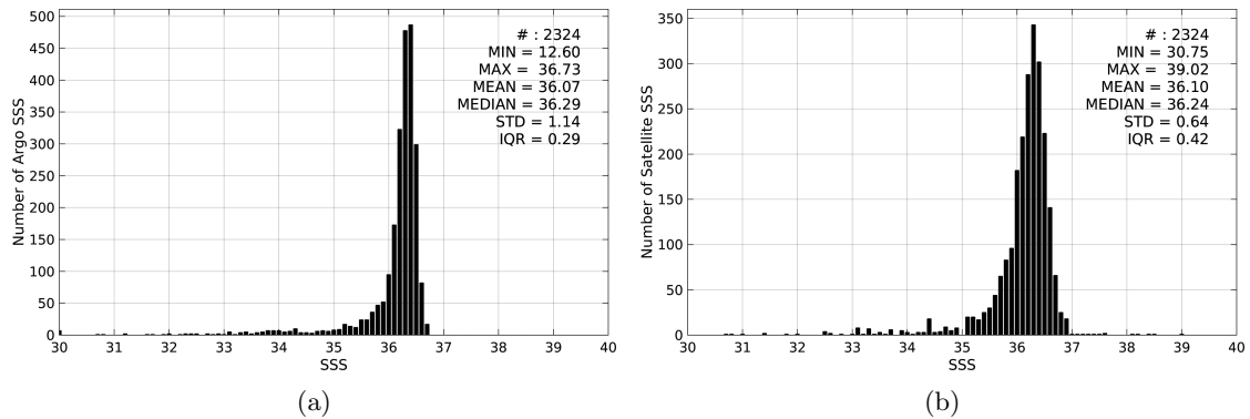
Figure 2: Histograms of SSS from Argo (a) and SMAP-L3-RSS-V2-MONTHLY-0.25DEG-40KM (b) considering all match-up pairs per bins of 0.1 over the Gulf of Mexico Pi-MEP region and for the full satellite product period.
