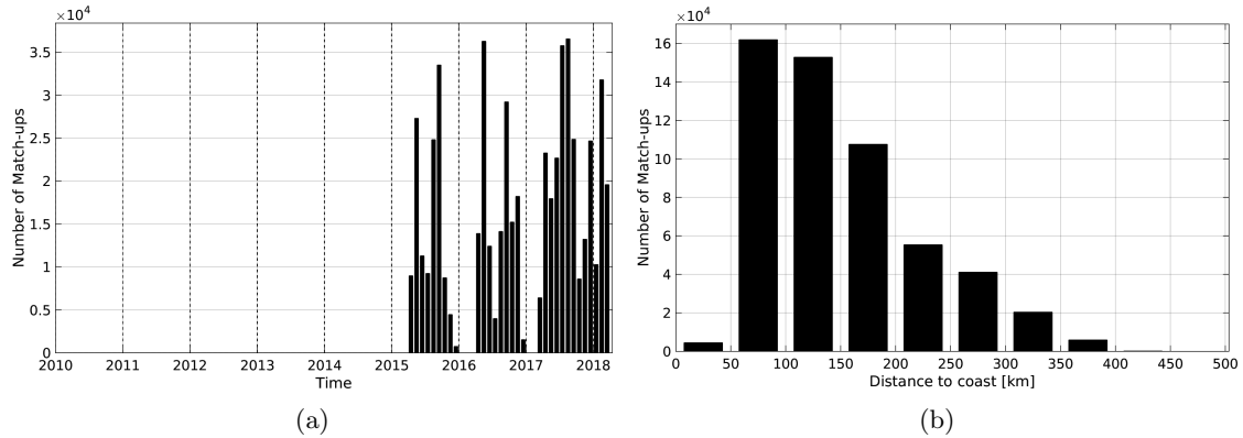
Figure 1: Number of match-ups between TSG-SAMOS and SMAP-L3-RSS-V2-MONTHLY-70KM SSS as a function of time (a) and as function of the distance to coast (b) over the Gulf of Mexico Pi-MEP region and for the full satellite product period.
