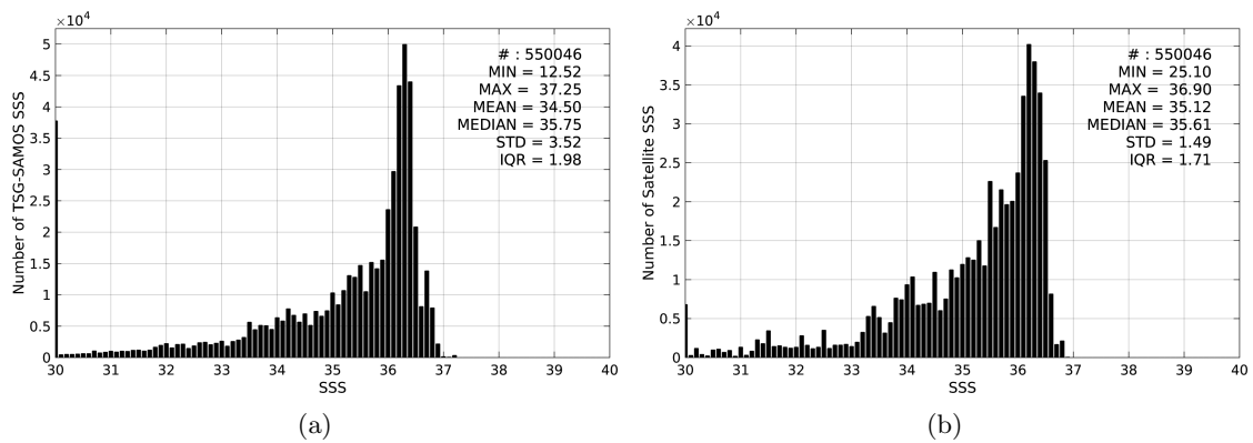
Figure 2: Histograms of SSS from TSG-SAMOS (a) and SMAP-L3-RSS-V2-MONTHLY-70KM (b) considering all match-up pairs per bins of 0.1 over the Gulf of Mexico Pi-MEP region and for the full satellite product period.
