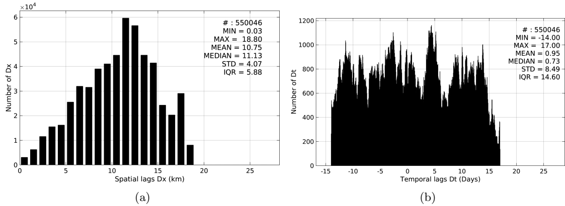
Figure 5: Histograms of the spatial (a) and temporal (b) lags between the time of the TSG-SAMOS measurements and the date of the corresponding SMAP-L3-RSS-V2-MONTHLY-70KM SSS product.
