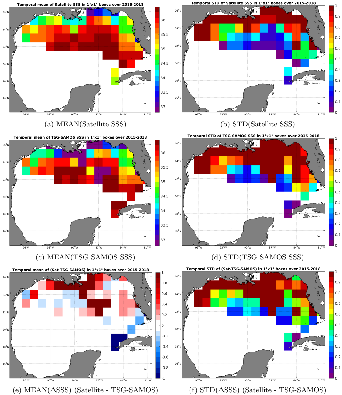
Figure 6: Temporal mean (left) and STD (right) of SSS from SMAP-L3-RSS-V2-MONTHLY-70KM (top), TSG-SAMOS (middle), and of \Delta SSS (Satellite - TSG-SAMOS). Only match-up pairs are used to generate these maps.
