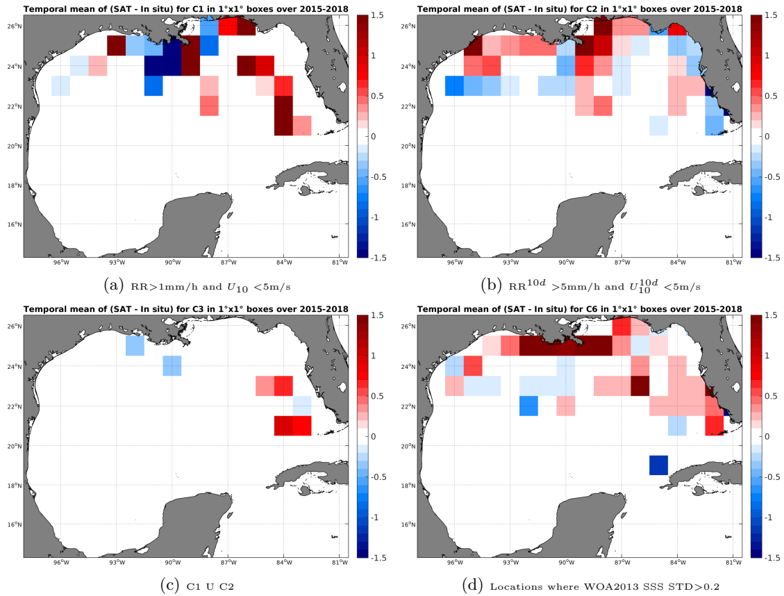
Figure 12: Temporal mean gridded over spatial boxes of size 1°x1° of \Delta SSS (SMAP-L3-RSS-V2-MONTHLY-70KM - TSG-SAMOS) for 4 different subdatasets corresponding to:RR>1mm/h and U_{10} < 5 m/s (a), RR^{10d} > 5 mm/h and U_{10}^{10d} < 5 m/s (b), C1 U C2 (c),Locations where WOA2013 SSS STD>0.2 (d).
