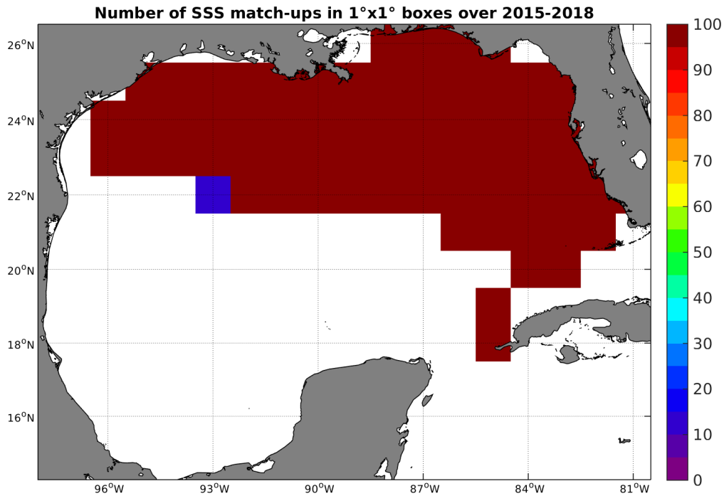
Figure 4: Number of SSS match-ups between TSG-SAMOS SSS and the SMAP-L3-RSS-V2-MONTHLY-70KM SSS product for the Gulf of Mexico Pi-MEP region over 1^\circ \times 1^\circ boxes and for the full satellite product period.
