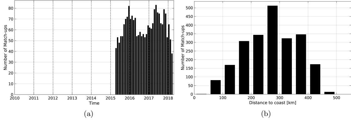
Figure 1: Number of match-ups between Argo and SMAP-L3-RSS-V2-MONTHLY-70KM SSS as a function of time (a) and as function of the distance to coast (b) over the Gulf of Mexico Pi-MEP region and for the full satellite product period.
