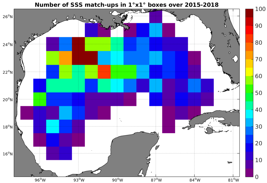
Figure 4: Number of SSS match-ups between Argo SSS and the SMAP-L3-RSS-V2-MONTHLY-70KM SSS product for the Gulf of Mexico Pi-MEP region over 1^\circ \times 1^\circ boxes and for the full satellite product period.
