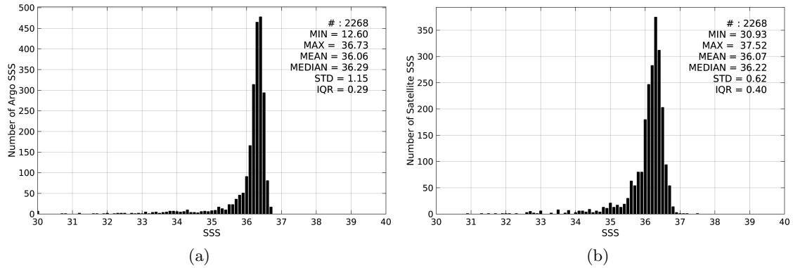
Figure 2: Histograms of SSS from Argo (a) and SMAP-L3-RSS-V2-MONTHLY-70KM (b) considering all match-up pairs per bins of 0.1 over the Gulf of Mexico Pi-MEP region and for the full satellite product period.
