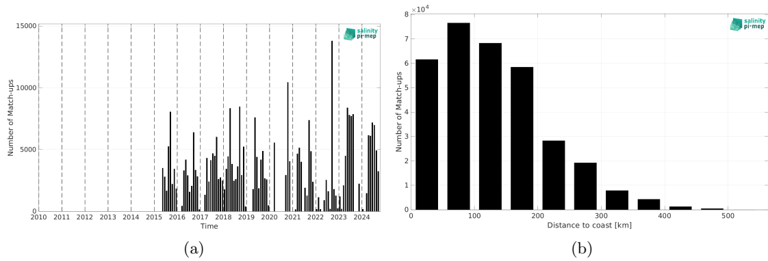
Figure 2: Number of match-ups between TSG (SAMOS) and SMAP SSS L3 v5.0 - 8-Day running (JPL) SSS as a function of time (a) and as function of the distance to coast (b) over the Gulf of Mexico Pi-MEP region and for the full satellite product period.
