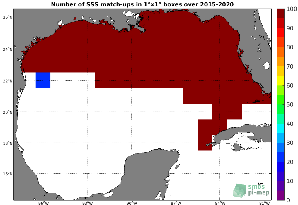
Figure 4: Number of SSS match-ups between TSG (SAMOS) SSS and the SMAP SSS L3 v5.0 - 8-Day running (JPL) SSS product for the Gulf of Mexico Pi-MEP region over 1°x1° boxes and for the full satellite product period.
