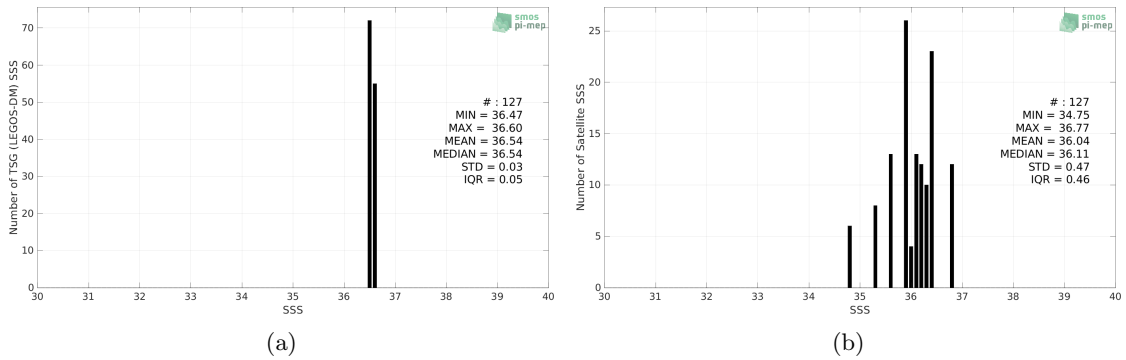
Figure 2: Histograms of SSS from TSG (LEGOS-DM) (a) and SMAP SSS L3 v5.0 - 8-Day running (JPL) (b) considering all match-up pairs per bins of 0.1 over the Gulf of Mexico Pi-MEP region and for the full satellite product period.
