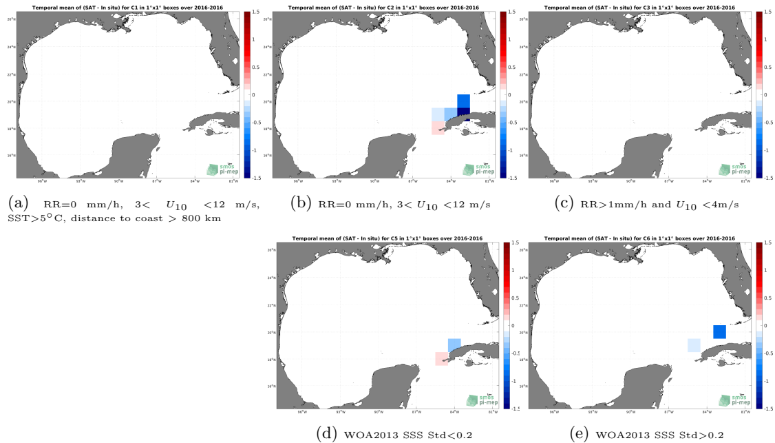
Figure 12: Temporal mean gridded over spatial boxes of size 1^{\circ}\times 1^{\circ} of \Delta\text{SSS} (SMAP SSS L3 v5.0 - 8-Day running (JPL) - TSG (LEGOS-DM)) for 5 different subdatasets corresponding to:RR=0 mm/h, 3 < U_{10} < 12 m/s, SST >5^{\circ}\text{C} , distance to coast > 800 km (a), RR=0 mm/h, 3 < U_{10} < 12 m/s (b), RR >1 mm/h and U_{10} < 4 m/s (c), WOA2013 SSS Std <0.2 (d), WOA2013 SSS Std >0.2 (e).
