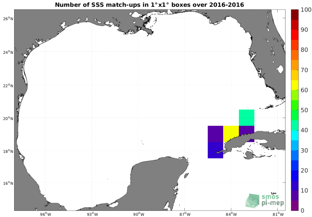
Figure 4: Number of SSS match-ups between TSG (LEGOS-DM) SSS and the SMAP SSS L3 v5.0 - 8-Day running (JPL) SSS product for the Gulf of Mexico Pi-MEP region over 1^\circ \times 1^\circ boxes and for the full satellite product period.
