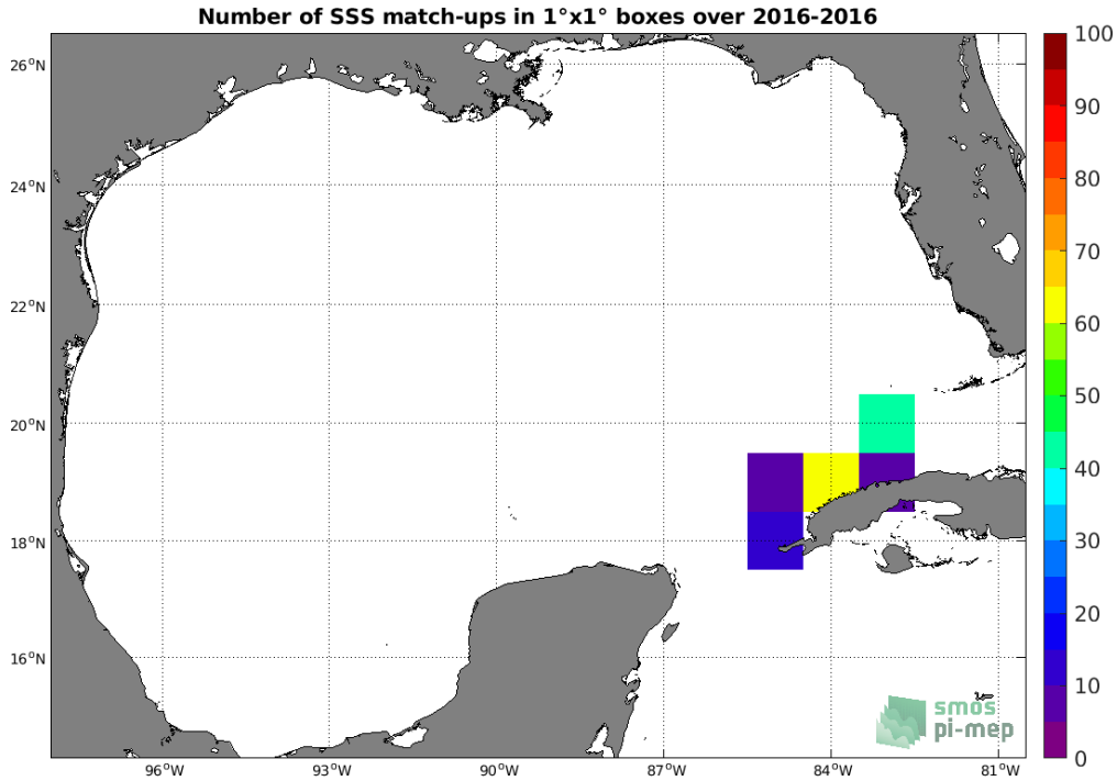
Figure 4: Number of SSS match-ups between TSG (LEGOS-DM) SSS and the SMAP SSS L3 v5.0 - 8-Day running (JPL) SSS product for the Gulf of Mexico Pi-MEP region over 1^{\circ} \times 1^{\circ} boxes and for the full satellite product period.
