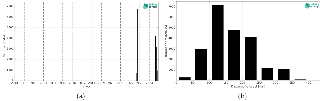
Figure 2: Number of match-ups between Saildrone and SMAP SSS L3 v5.0 - 8-Day running (JPL) SSS as a function of time (a) and as function of the distance to coast (b) over the Gulf of Mexico Pi-MEP region and for the full satellite product period.
