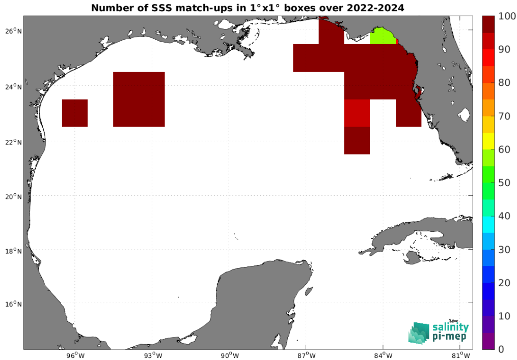
Figure 5: Number of SSS match-ups between Saildrone SSS and the SMAP SSS L3 v5.0 - 8-Day running (JPL) SSS product for the Gulf of Mexico Pi-MEP region over 1^\circ \times 1^\circ boxes and for the full satellite product period.
