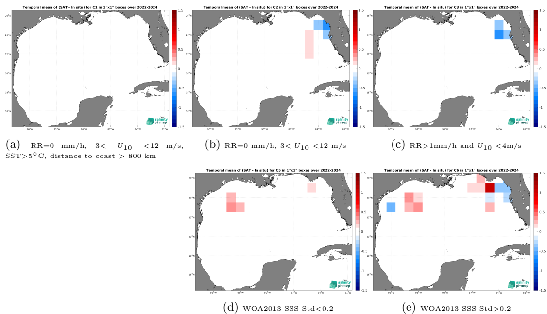
Figure 14: Temporal mean gridded over spatial boxes of size 1^\circ \times 1^\circ of \Delta\text{SSS} (SMAP SSS L3 v5.0 - 8-Day running (JPL) - Sairdron) for 5 different subdatasets corresponding to:RR=0 mm/h, 3 < U_{10} < 12 m/s, SST>5°C, distance to coast > 800 km (a), RR=0 mm/h, 3 < U_{10} < 12 m/s (b), RR>1mm/h and U_{10} < 4 m/s (c), WOA2013 SSS Std<0.2 (d), WOA2013 SSS Std>0.2 (e).
