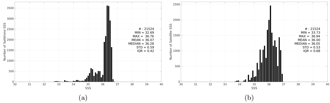
Figure 3: Histograms of SSS from Saildrone (a) and SMAP SSS L3 v5.0 - 8-Day running (JPL) (b) considering all match-up pairs per bins of 0.1 over the Gulf of Mexico Pi-MEP region and for the full satellite product period.
