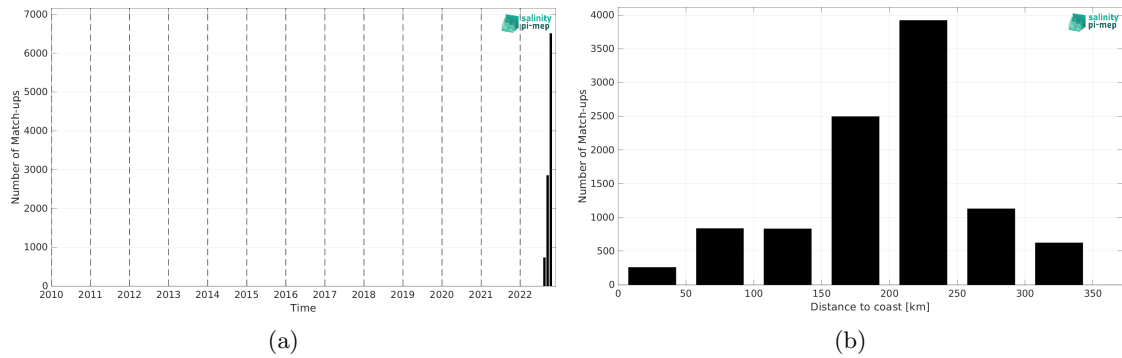
Figure 1: Number of match-ups between Sairdrone and SMAP SSS L3 v5.0 - 8-Day running (JPL) SSS as a function of time (a) and as function of the distance to coast (b) over the Gulf of Mexico Pi-MEP region and for the full satellite product period.
