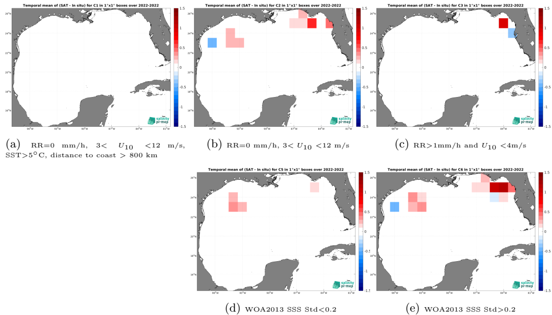
Figure 12: Temporal mean gridded over spatial boxes of size 1^{\circ}\times 1^{\circ} of \Delta\text{SSS} (SMAP SSS L3 v5.0 - 8-Day running (JPL) - Sailydrone) for 5 different subdatasets corresponding to:RR=0 mm/h, 3 < U_{10} < 12 m/s, SST >5^{\circ}\text{C} , distance to coast > 800 km (a), RR=0 mm/h, 3 < U_{10} < 12 m/s (b), RR >1 mm/h and U_{10} < 4 m/s (c), WOA2013 SSS Std <0.2 (d), WOA2013 SSS Std >0.2 (e).
