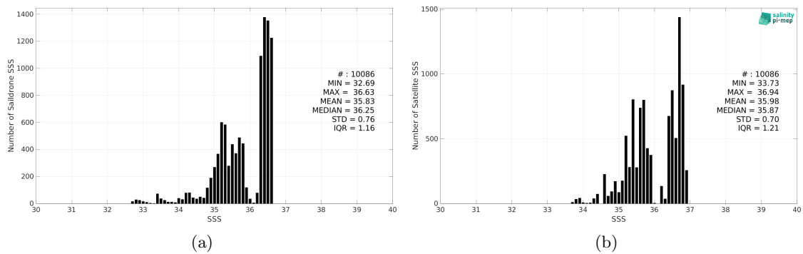
Figure 2: Histograms of SSS from Sairdrone (a) and SMAP SSS L3 v5.0 - 8-Day running (JPL) (b) considering all match-up pairs per bins of 0.1 over the Gulf of Mexico Pi-MEP region and for the full satellite product period.
