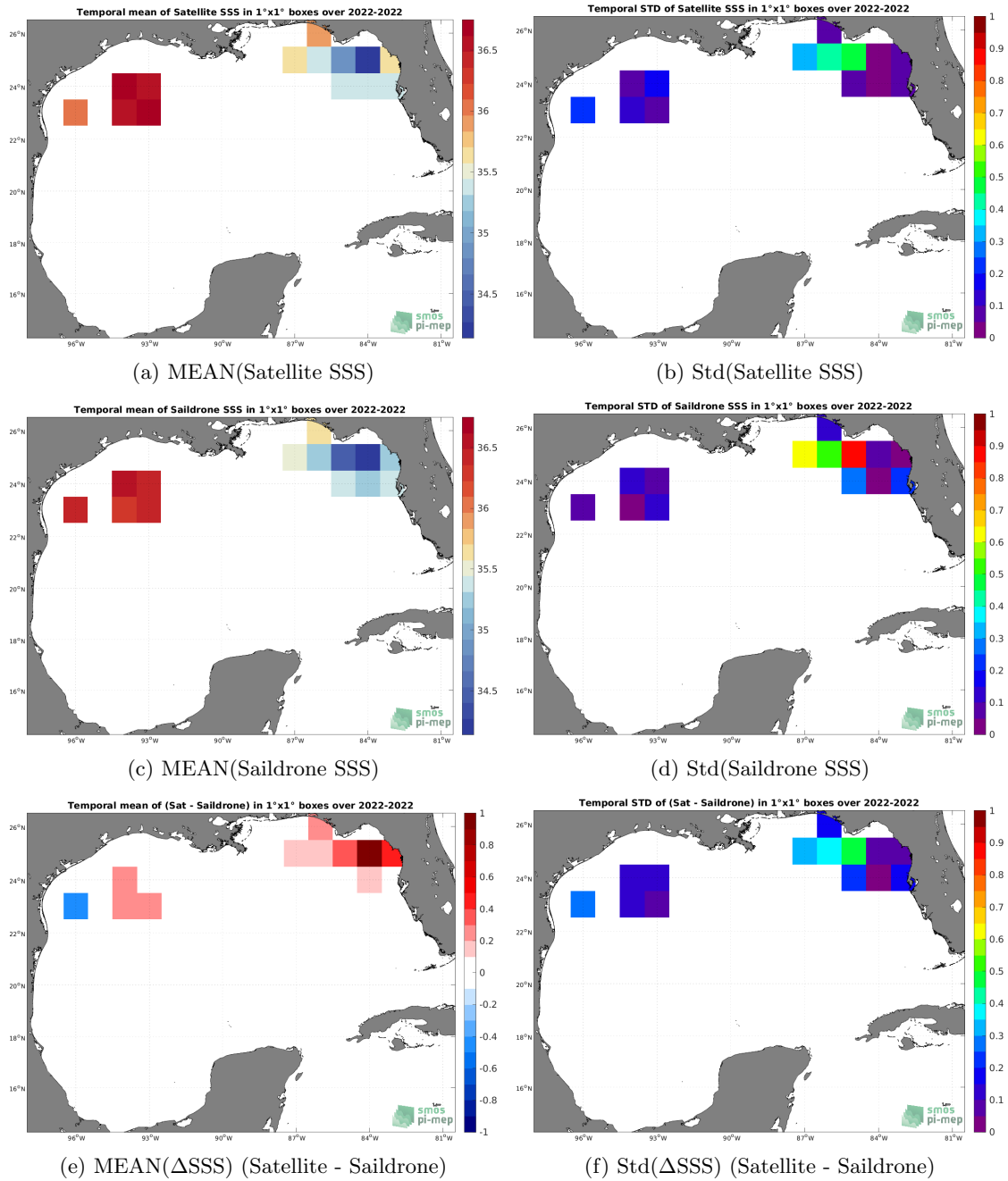
Figure 6: Temporal mean (left) and Std (right) of SSS from SMAP SSS L3 v5.0 - 8-Day running (JPL) (top), Saildrone (middle), and of \Delta SSS (Satellite - Saildrone). Only match-up pairs are used to generate these maps.
