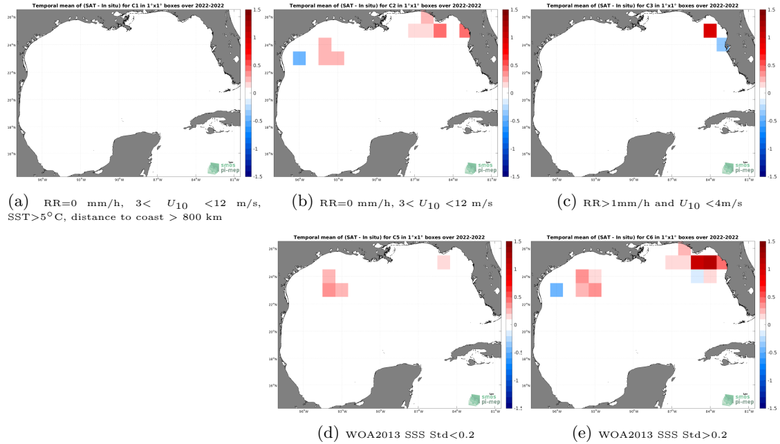
Figure 12: Temporal mean gridded over spatial boxes of size 1^{\circ}\times 1^{\circ} of \Delta\text{SSS} (SMAP SSS L3 v5.0 - 8-Day running (JPL) - Sairdrone) for 5 different subdatasets corresponding to:RR=0 mm/h, 3 < U_{10} < 12 m/s, SST >5^{\circ}\text{C} , distance to coast > 800 km (a), RR=0 mm/h, 3 < U_{10} < 12 m/s (b), RR >1 mm/h and U_{10} < 4 m/s (c), WOA2013 SSS Std <0.2 (d), WOA2013 SSS Std >0.2 (e).
