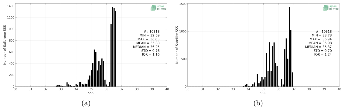
Figure 2: Histograms of SSS from Saildrone (a) and SMAP SSS L3 v5.0 - 8-Day running (JPL) (b) considering all match-up pairs per bins of 0.1 over the Gulf of Mexico Pi-MEP region and for the full satellite product period.
