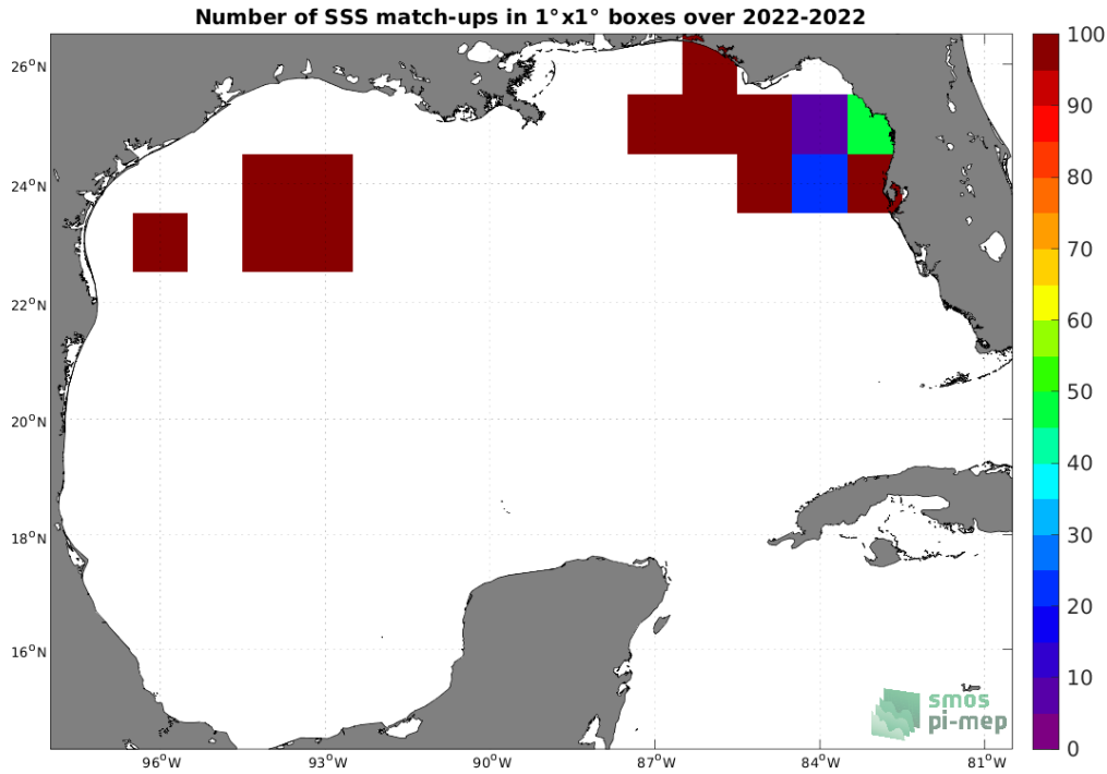
Figure 4: Number of SSS match-ups between Saildrone SSS and the SMAP SSS L3 v5.0 - 8-Day running (JPL) SSS product for the Gulf of Mexico Pi-MEP region over 1^\circ \times 1^\circ boxes and for the full satellite product period.
