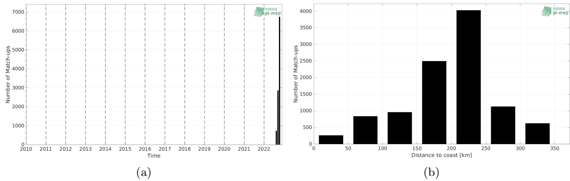
Figure 1: Number of match-ups between Saildrone and SMAP SSS L3 v5.0 - 8-Day running (JPL) SSS as a function of time (a) and as function of the distance to coast (b) over the Gulf of Mexico Pi-MEP region and for the full satellite product period.
