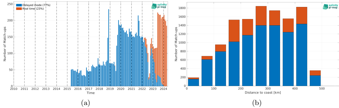
Figure 2: Number of match-ups between Argo and SMAP SSS L3 v5.0 - 8-Day running (JPL) SSS as a function of time (a) and as function of the distance to coast (b) over the Gulf of Mexico Pi-MEP region and for the full satellite product period.
