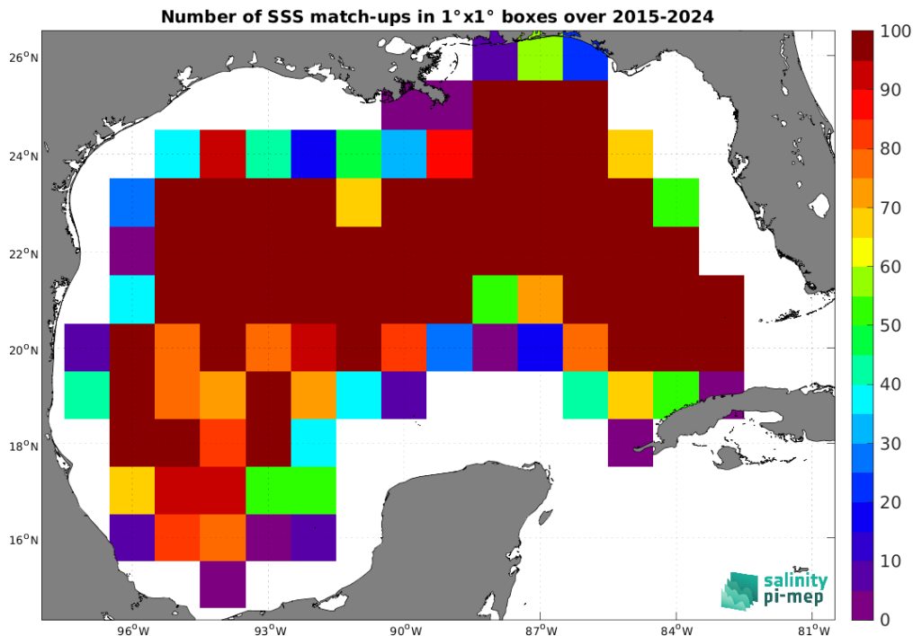
Figure 5: Number of SSS match-ups between Argo SSS and the SMAP SSS L3 v5.0 - 8-Day running (JPL) SSS product for the Gulf of Mexico Pi-MEP region over 1^\circ \times 1^\circ boxes and for the full satellite product period.
