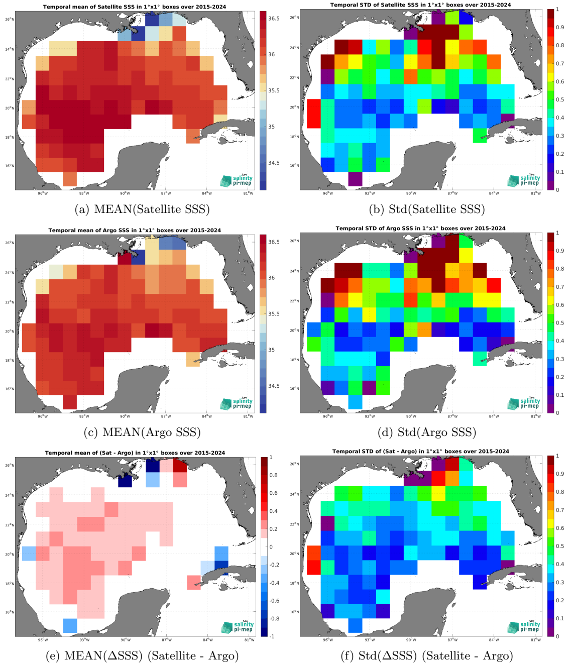
Figure 7: Temporal mean (left) and Std (right) of SSS from SMAP SSS L3 v5.0 - 8-Day running (JPL) (top), Argo (middle), and of \Delta SSS (Satellite - Argo). Only match-up pairs are used to generate these maps.
