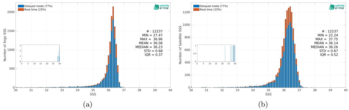
Figure 3: Histograms of SSS from Argo (a) and SMAP SSS L3 v5.0 - 8-Day running (JPL) (b) considering all match-up pairs per bins of 0.1 over the Gulf of Mexico Pi-MEP region and for the full satellite product period.
