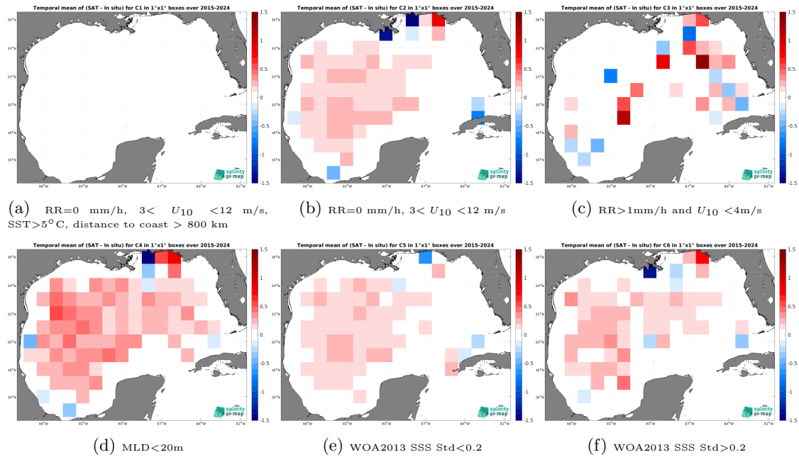
Figure 14: Temporal mean gridded over spatial boxes of size 1^\circ \times 1^\circ of \Delta\text{SSS} (SMAP SSS L3 v5.0 - 8-Day running (JPL) - Argo) for 6 different subdatasets corresponding to:RR=0 mm/h, 3 < U_{10} < 12 m/s, SST > 5°C, distance to coast > 800 km (a), RR=0 mm/h, 3 < U_{10} < 12 m/s (b), RR > 1mm/h and U_{10} < 4 m/s (c),MLD < 20m (d),WOA2013 SSS Std < 0.2 (e),WOA2013 SSS Std > 0.2 (f).
