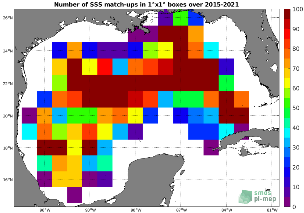
Figure 4: Number of SSS match-ups between Argo SSS and the SMAP SSS L3 v5.0 - 8-Day running (JPL) SSS product for the Gulf of Mexico Pi-MEP region over 1°x1° boxes and for the full satellite product period.
