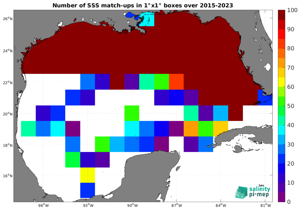
Figure 5: Number of SSS match-ups between TSG (SAMOS) SSS and the SMAP SSS L3 v5.0 - Monthly (JPL) SSS product for the Gulf of Mexico Pi-MEP region over 1°x1° boxes and for the full satellite product period.
