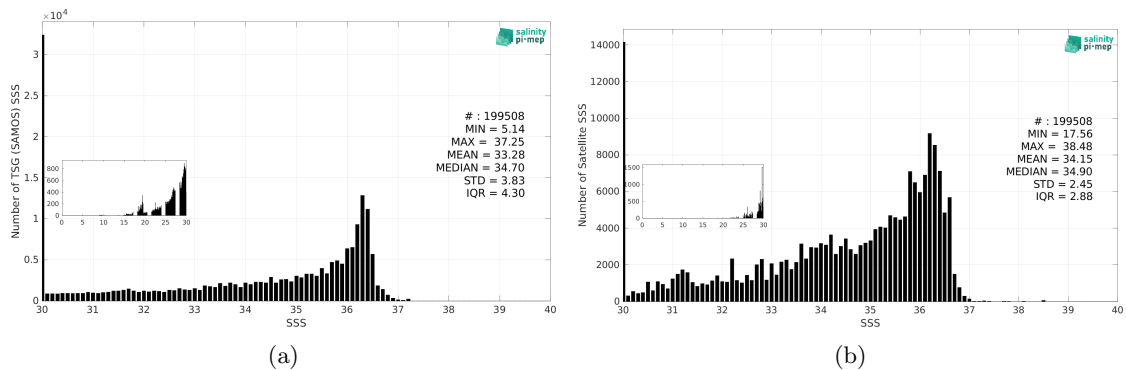
Figure 3: Histograms of SSS from TSG (SAMOS) (a) and SMAP SSS L3 v5.0 - Monthly (JPL) (b) considering all match-up pairs per bins of 0.1 over the Gulf of Mexico Pi-MEP region and for the full satellite product period.
