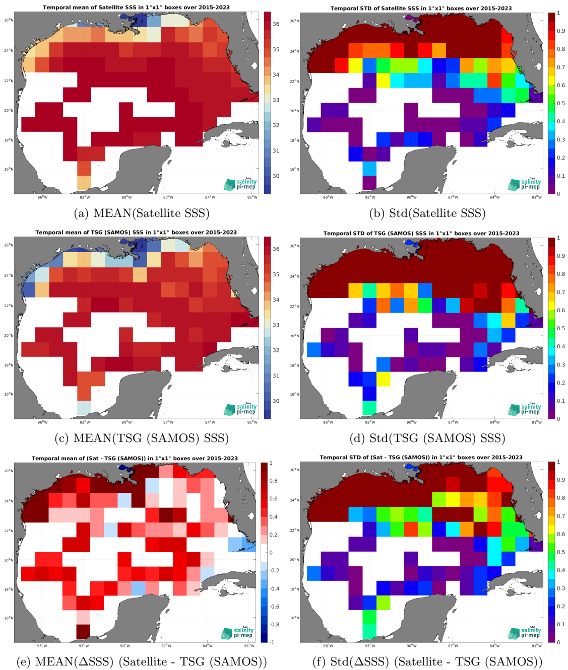
Figure 7: Temporal mean (left) and Std (right) of SSS from SMAP SSS L3 v5.0 - Monthly (JPL) (top), TSG (SAMOS) (middle), and of \Delta SSS (Satellite - TSG (SAMOS)). Only match-up pairs are used to generate these maps.
