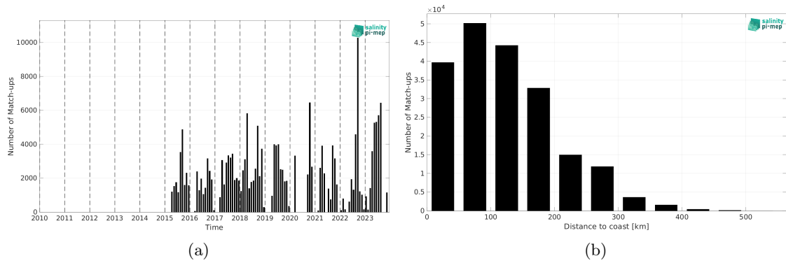
Figure 2: Number of match-ups between TSG (SAMOS) and SMAP SSS L3 v5.0 - Monthly (JPL) SSS as a function of time (a) and as function of the distance to coast (b) over the Gulf of Mexico Pi-MEP region and for the full satellite product period.
