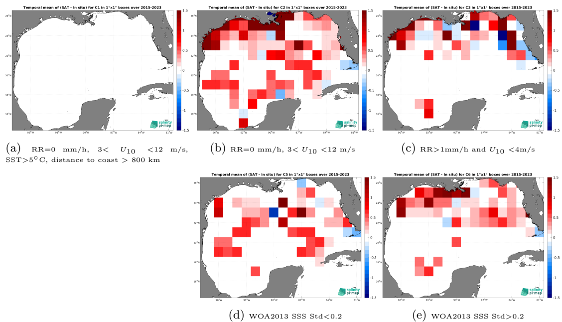
Figure 14: Temporal mean gridded over spatial boxes of size 1^\circ \times 1^\circ of \Delta\text{SSS} (SMAP SSS L3 v5.0 - Monthly (JPL) - TSG (SAMOS)) for 5 different subdatasets corresponding to:RR=0 mm/h, 3 < U_{10} < 12 m/s, SST >5^\circ\text{C} , distance to coast > 800 km (a), RR=0 mm/h, 3 < U_{10} < 12 m/s (b), RR >1 mm/h and U_{10} < 4 m/s (c), WOA2013 SSS Std <0.2 (d), WOA2013 SSS Std >0.2 (e).
